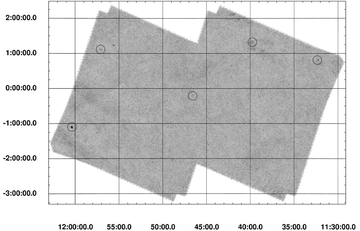
Fig. 2. Positions of the ERCSC 857 GHz sources in the 350 \mu m H-ATLAS GAMA-12 field.
