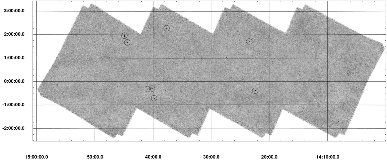
Fig. 3. Positions of the ERCSC 857 GHz sources in the 350 \mu m H-ATLAS GAMA-15 field.
