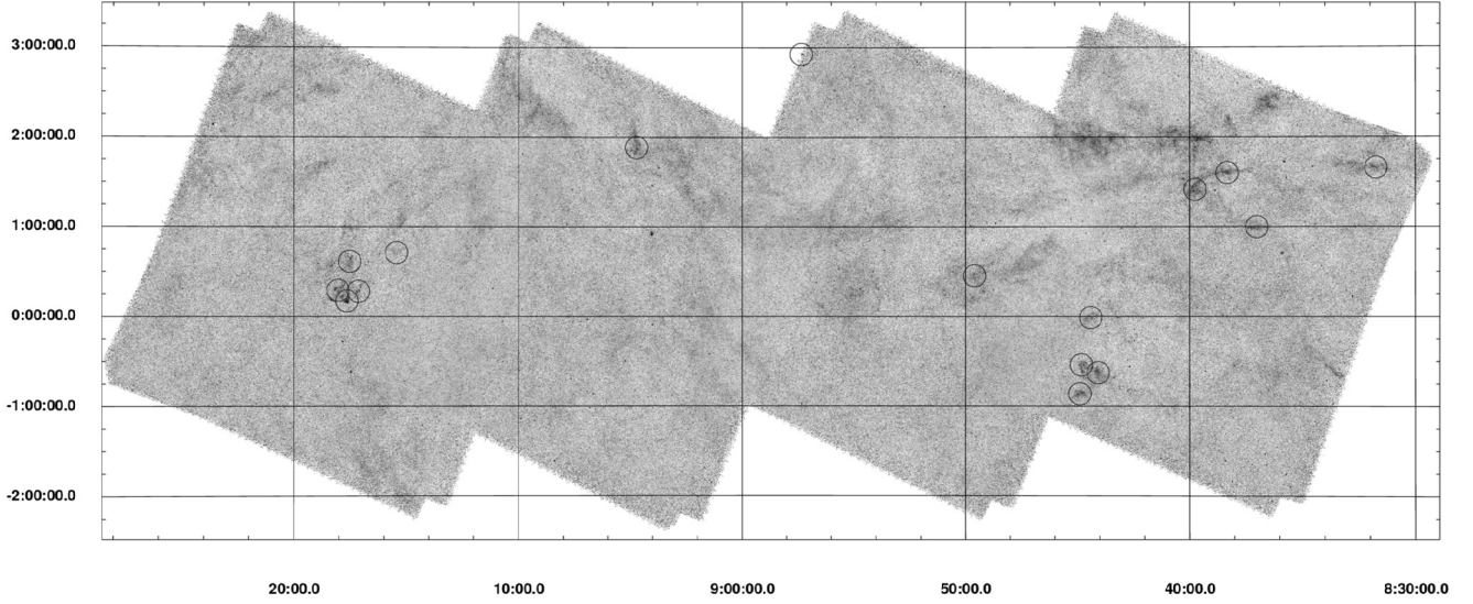
Fig. 1. Positions of the ERCSC 857 GHz sources in the 350 \mu m H-ATLAS GAMA-09 field. The source at coordinates 0857+3 has not been included in this analysis because it lies on the poorly sampled edge of the field.
