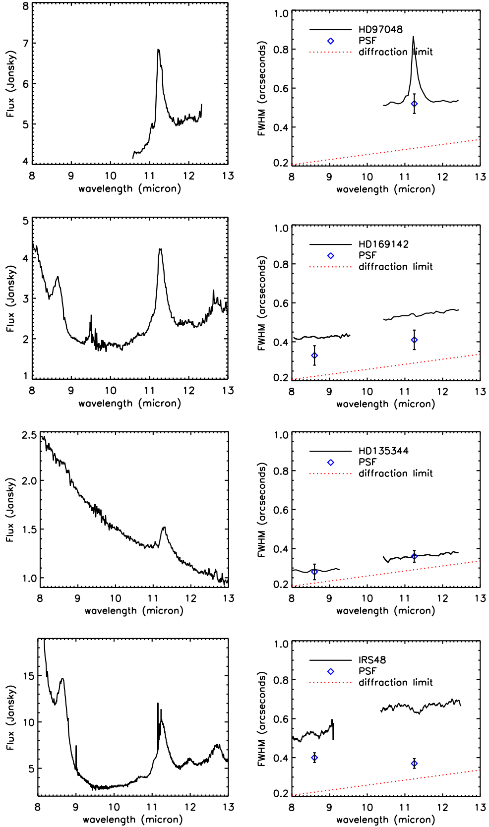
Fig. 2. VISIR observations in the N -band. Left: the observed spectra, right: the corresponding FWHM (in arcseconds) as a function of wavelength. From top to bottom, the VISIR observations of HD 97048, HD 169142, HD 135344 B, and Oph IRS 48 are shown. The red line shows the diffraction limit for a 8.2 m telescope; the blue diamonds show the PSF values of the statistical calibrator. The 11.2 \mu\text{m} PAH feature in HD 97048 is more extended than the continuum (which is unresolved) and as large as the continuum for HD 169142, but smaller than the continuum in Oph IRS 48. For HD 135344 B, the continuum and PAH features are both unresolved.
