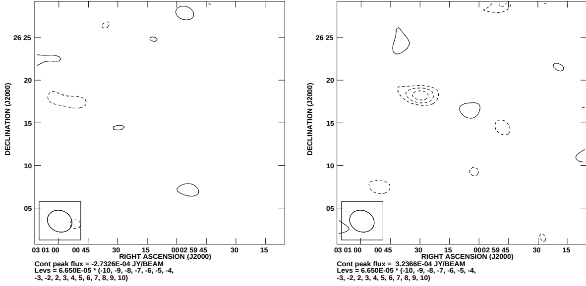
Figure 3. The jack-knifed SA pointed observations of the cluster candidate (an image of the data is shown on the left of Figure 6). On the left, data are split into plus and minus baseline, on the right, data are split according to median date. The contour levels are linear from 2 \sigma_{SA,survey} to 10 \sigma_{SA,survey} ( \sigma_{SA,pointed} = 65 \mu Jy ); positive contours are solid lines and negative contours are dashed lines. The ellipse at the bottom left of the maps shows the SA synthesised beam.
