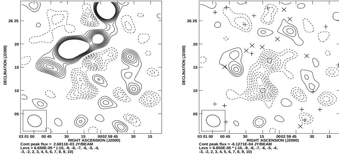
Figure 6. The AMI SA pointed observation towards the cluster. On the left is the map before source-subtraction and on the right is the map after the relevant sources in Table 5 have been subtracted. The + symbols indicate the positions of sources with flux densities less than 4\sigma_{\text{SA,pointed}} on the SA map. For this run, the sampler has been allowed to fit the positions of the × type sources with a Gaussian centred on the LA source position. The contour levels are linear from 2\sigma_{\text{SA,pointed}} to 10\sigma_{\text{SA,pointed}} ( \sigma_{\text{SA,pointed}} = 65\mu\text{Jy} ); positive contours are solid lines and negative contours are dashed lines. The boxes indicate the positions of the cluster candidates. Candidate 1 is at J 03 h 00 m 14.8 s +26° 10′ 02.6″ and candidate 2 is at J 03 h 00 m 08.9 s +26° 16′ 29.1″. When imaging the source subtracted map CLEAN boxes have been placed around each candidate. The ellipse at the bottom left of the maps shows the SA synthesised beam.
