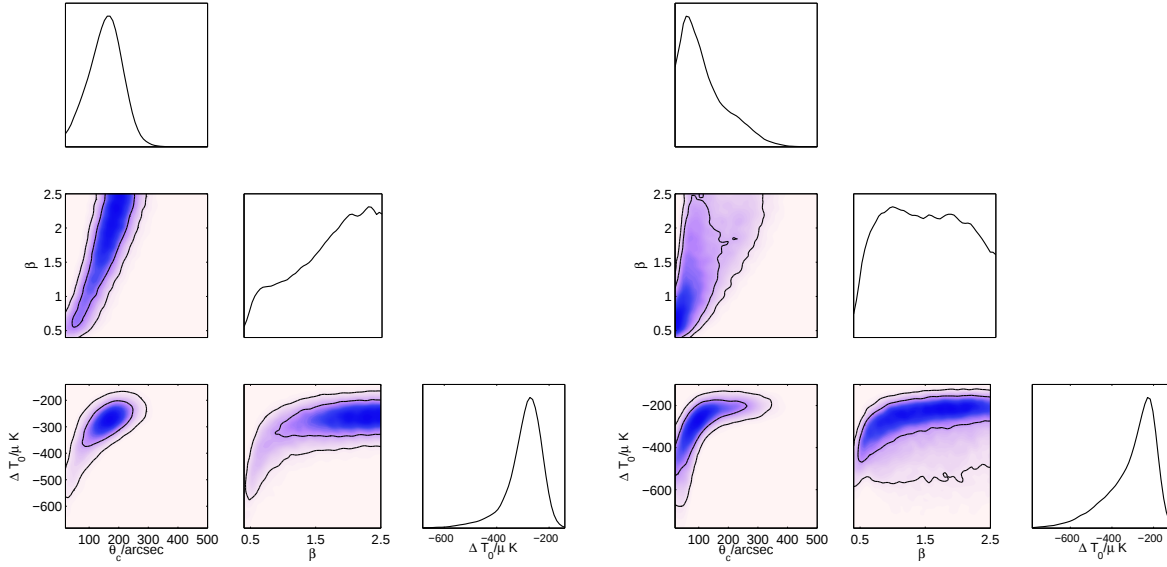
Figure 9. 1D and 2D marginal posterior distributions for the parameters in the SZ decrement model for candidate 1 (left) and candidate 2 (right).
