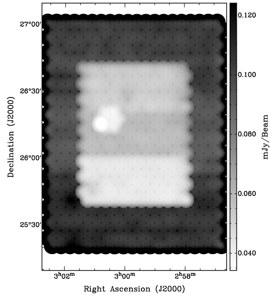
Figure 1. Noise map for the LA survey field. The inner region noise is \approx 50\mu\text{Jy} , while the noise on the outer region is \approx 100\mu\text{Jy} . The hexagonal region around 03^{\text{h}} 00^{\text{m}} 10^{\text{s}} +26^{\circ} 15' 00'' is next to the cluster and was observed to \approx 30\mu\text{Jy} . The inner region of the noise map consists of three subregions; these have slightly different sensitivities due to varying weather conditions and slight differences in observing time.
