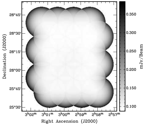
Figure 2. Noise map for the SA AMI002 field. The noise at the edge of the map increases due to the primary beam of the SA. In the central region the map noise is \approx 100\mu\text{Jy} . This noise map does not include the follow-up SA observations towards 03^{\text{h}}00^{\text{m}}08.66^{\text{s}} +26^{\circ}15'16.1'' as those data were analysed separately. The noise level of the follow-up SA observations is 65\mu\text{Jy} .
