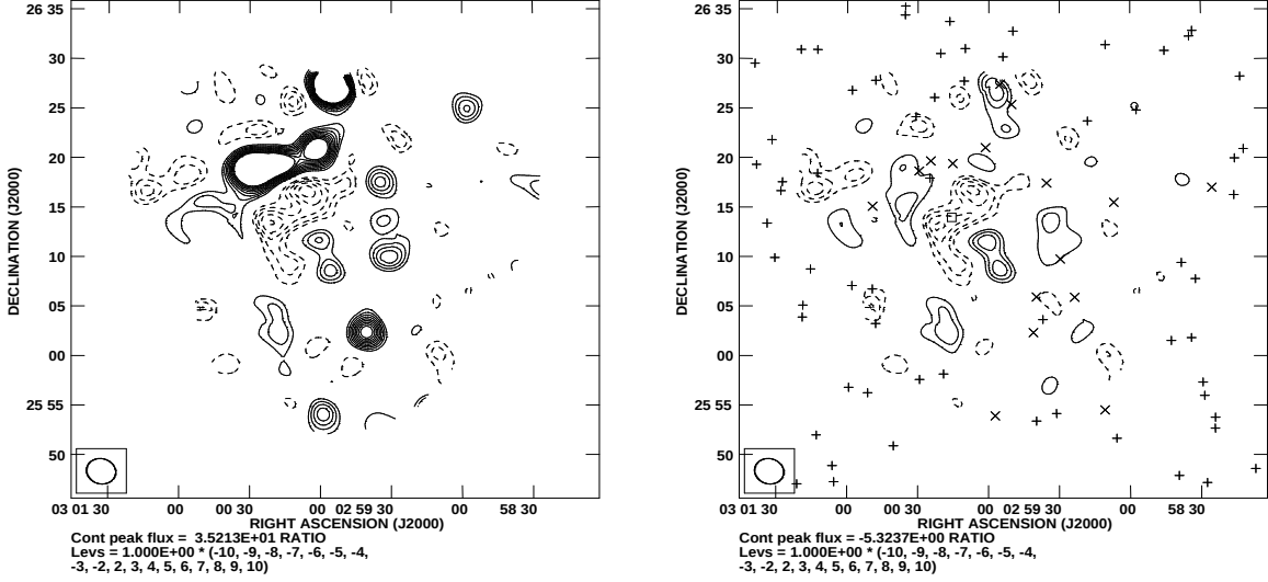
Figure 5. The SA survey-field observations of the cluster candidate. On the left is the map before source subtraction and on the right is after the map after the sources in Table 5 have been subtracted. The + symbols indicate the positions of sources with flux densities less than 4 \sigma_{\text{SA,survey}} and the \times symbols represent sources which have a flux density greater than 4 \sigma_{\text{SA,survey}} . The box on the source-subtracted map shows the position of the cluster candidate. These maps are signal-to-noise maps. Each pointing has a thermal-noise level of approximately 0.11 mJy. The contour levels are linear from 2 \sigma_{\text{SA,survey}} to 10 \sigma_{\text{SA,survey}} ; positive contours are solid lines and negative contours are dashed lines. The ellipse at the bottom left of the maps shows the SA synthesised beam.
