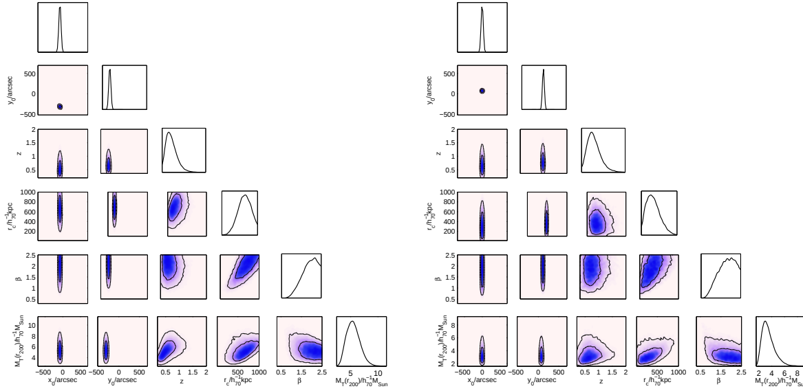
Figure 8. 1D and 2D marginal posterior distributions for a selection of the parameters in physical cluster model for candidate 1 (left) and candidate 2 (right). The M_{T,200} values have been divided by 10^{14} .
