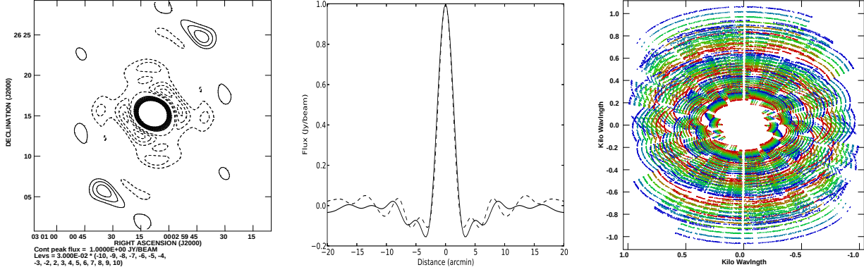
Figure 7. On the left is the synthesized beam for the AMI SA pointed observation towards the cluster (Figure 6). The contour levels range from 6% to 30% with intervals of 3%; positive contours are solid lines and negative contours are dashed lines. The image in the centre shows one-dimensional slices through the centre of the synthesised beam; dashed lines show the profile along the declination axis and solid lines show the profile along the right ascension axis. The image on the right shows the corresponding uv coverage of the observation; a different colour is used for each AMI channel.
