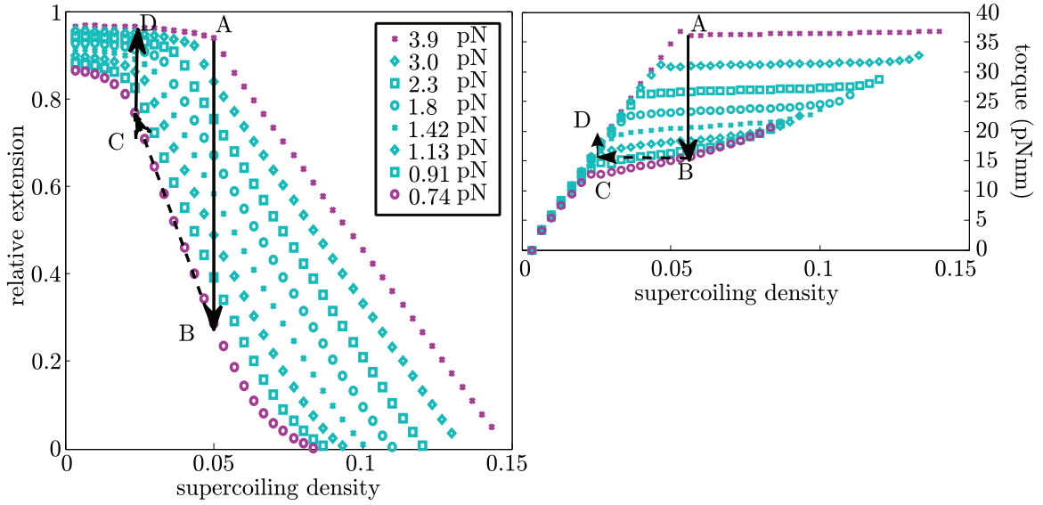
FIG. 12. (Color online) Illustration of the magnetic tweezer measurements from Mosconi et al. [37] as a basis for indirect torque measurements. The curves are calculated from our model for a range of tensions where fluctuations are small enough, using the criterion K^2 \geq 3 . The contour length is 5.6 \mu\text{m} and the monovalent salt concentration is 100 mM. On the left are the resulting turn-extension plots. On the right are torques from our model. Notice how the torque is increasing in the plectoneme region, caused by the growing number of plectonemes. The circuit ABCD results in too high a torque at C when one assume the plectoneme torque to be constant.
