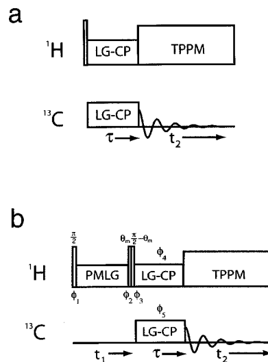
FIG. 1. Pulse sequences for 2D LG-CP (a) and 3D LG-CP (b) experiments. The phases of the 3D LG-CP experiment were \phi_1=x , \phi_2=y , \phi_3=-y , \phi_4=x , and \phi_5=x . The phases of the pre-LG-CP pulse ( \phi_3 ) and the LG-CP proton locking pulse ( \phi_4 ) were incremented according to the TPPI scheme.
