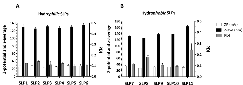
Figure 4: Physicochemical properties of the liposomal formulations loaded with (A) hydrophilic and (B) hydrophobic SLPs. Data are average \pm SD of 3 independent batches. ZP = zeta-potential measured in mV, Z-ave = Z-average particle diameter in nanometres, PDI = polydispersity index.
