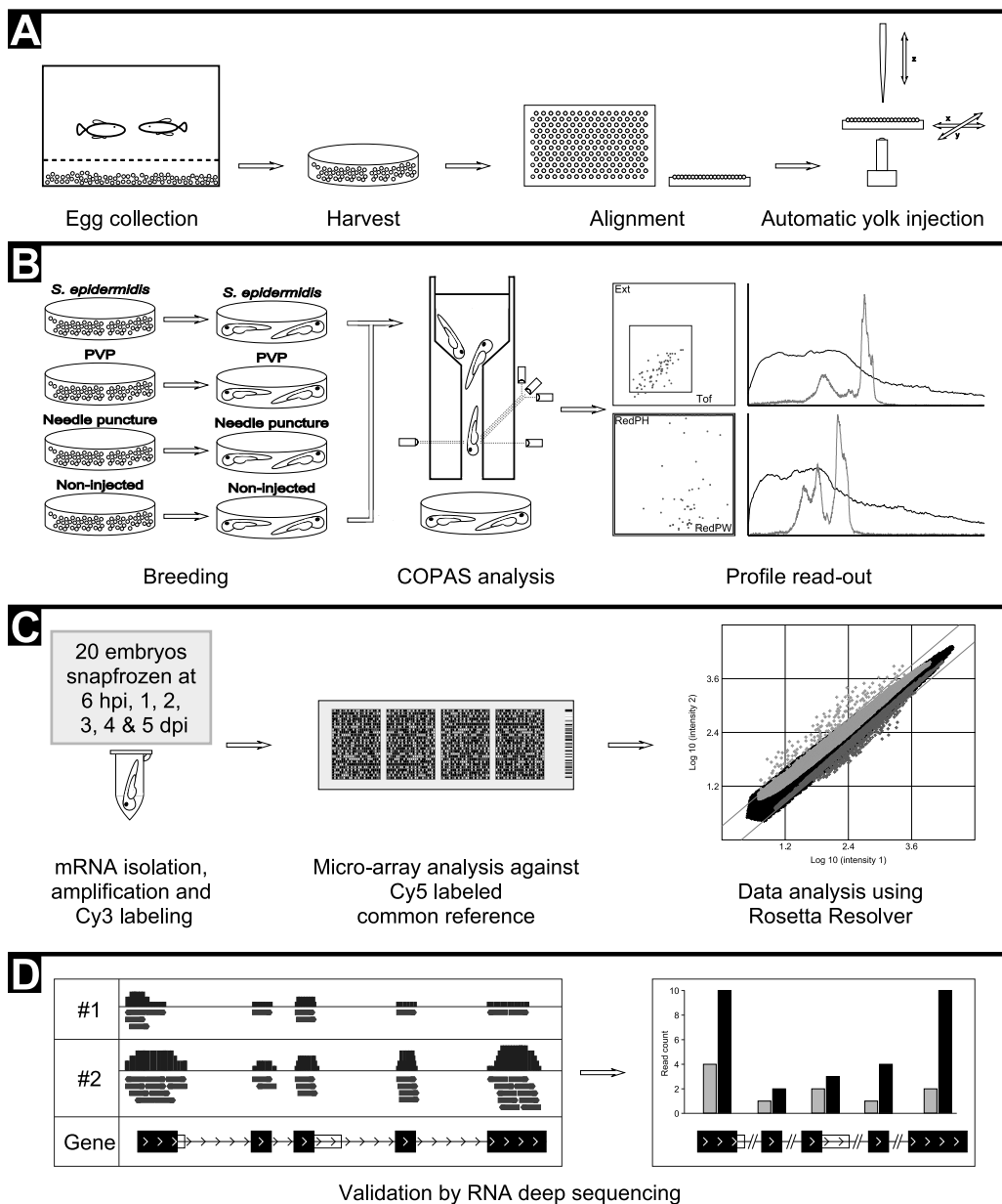
Figure 3. Workflow of high-throughput injection and subsequent analysis. (A) from left to right; a zebrafish pair are put together to mate, eggs are collected, eggs are distribute into a 1024 well agarose grid, eggs are injected into the yolk at 2 hpf using the automated micro-injection system. (B) from left to right; after injection, eggs are collected into Petri dishes and incubated at 28°C for a period of 5 days, COPAS analysis is performed on the S. epidermidis and non-injected embryos at 2, 3, 4 and 5 dpi. (C) from left to right; from all groups 20 embryos are snap frozen at 6 hpi, 1, 2, 3, 4 and 5 dpi for RNA isolation, amplification and Cy3 labelling, micro-array analysis against Cy5 labelled common reference and data analysis using Rosetta Resolver. (D) from left to right; validation of micro-array data was performed by RNAseq analysis of 4 biological replicas of S. epidermidis infected embryos at 5 dpi.
