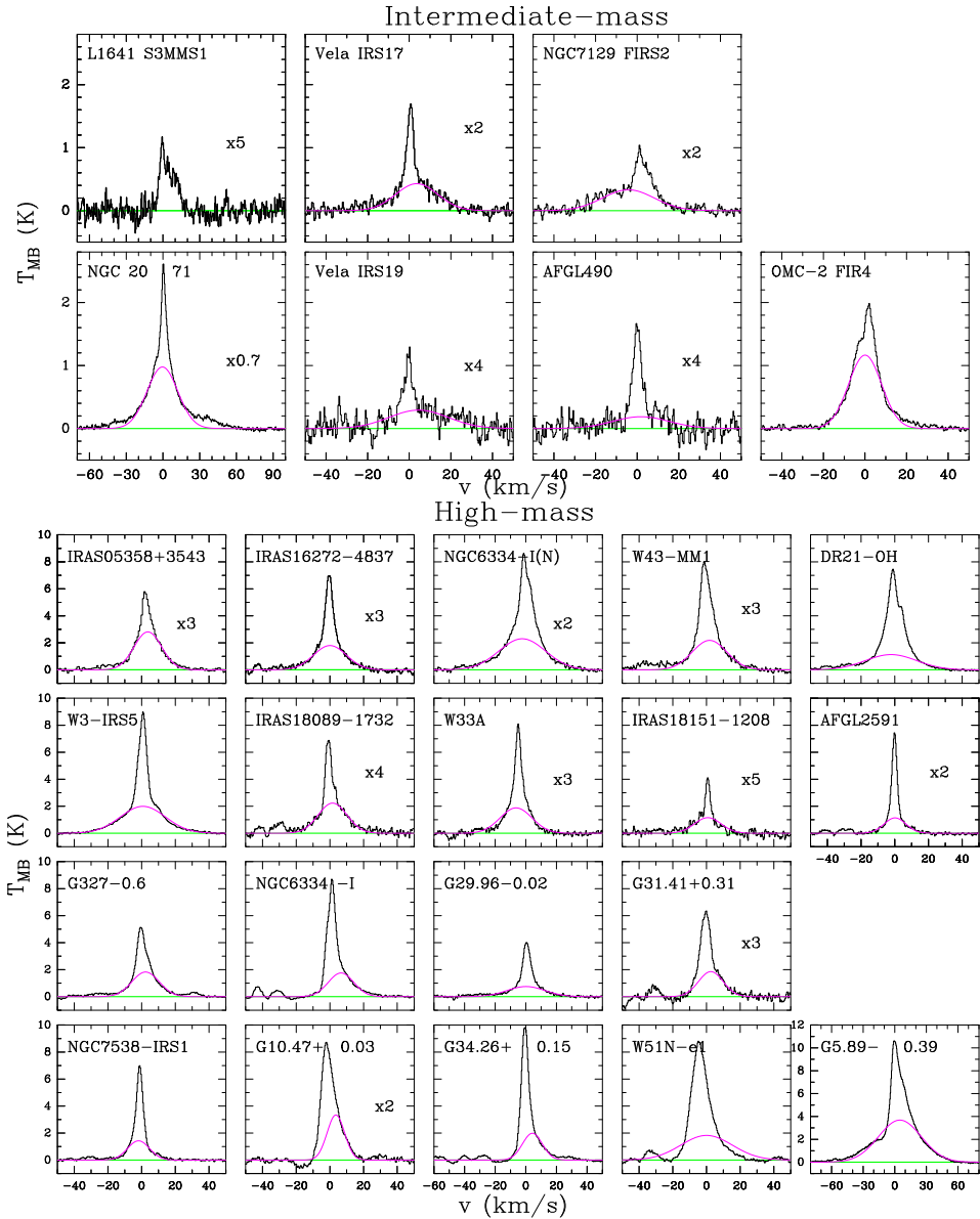
Figure 4.12: \text{H}_2\text{O } 2_{11}\text{-}2_{02} spectra for the intermediate-mass YSOs ( top ) and high-mass sources ( bottom ). The green line represents the baseline level and the pink Gaussian the broad velocity component. All spectra have been shifted to zero velocity. The numbers indicate where the spectra have been scaled for greater visibility.
