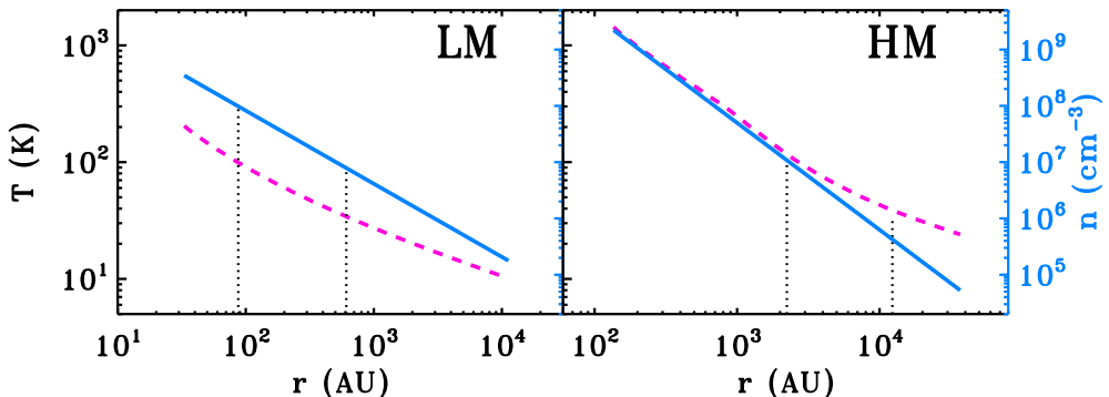
Figure 1.4: Temperature ( T , pink dashed line) and density profiles ( n , blue solid line) of a low-mass (LM; left ) and a high-mass (HM; right ) YSO as a function of the radius of the modelled envelope (distance from the central star). The vertical black dotted lines indicate the radii at which the gas and dust temperature reaches 100 and 35 K respectively.
