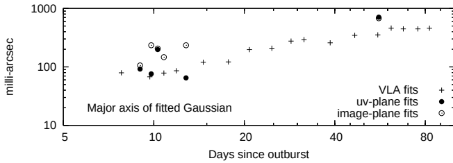
Figure 5. Expansion of the SGR 1806-20 radio source: a comparison of the major axes of the MERLIN and VLBA Gaussian fits (table 2) with fits to the VLA data from Taylor et al. (2005).
