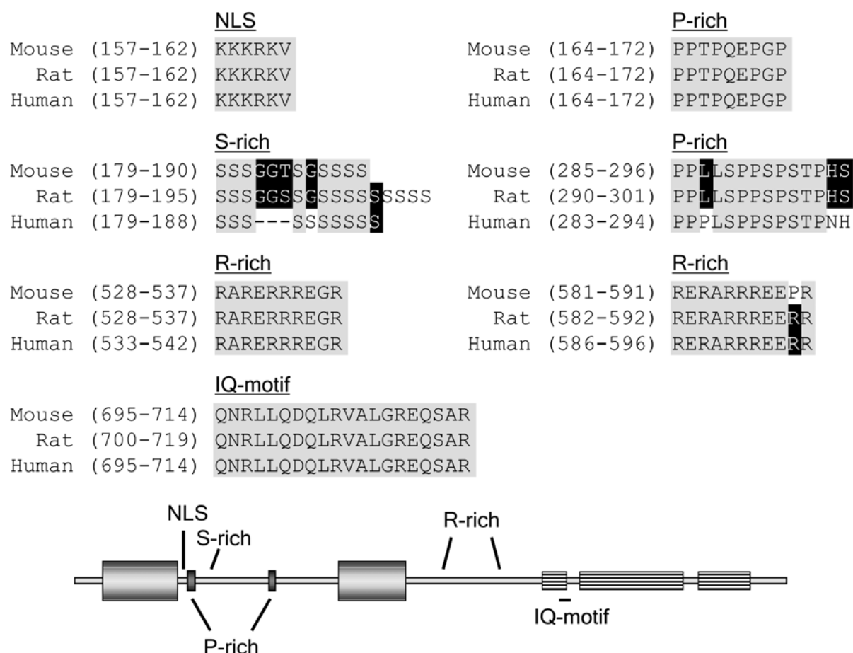
Figure 10. Conserved domains and putative interaction motifs of p116 Rip
