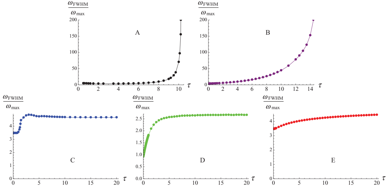
FIG. 7. (Color online) Peak width crossover. Evolution of the relative peak width, i.e., the ratio of the full width at half maximum (FWHM) of the peak and peak location \omega_{\text{max}} , as a function of reduced temperature \tau = (T - T_c)/T_c for the five different models. For FLBCS (case A) and CGBCS (case B), the ratio diverges at high temperature. For QCBCS (case C) there is a sudden change from the low-temperature relaxational behavior to the high-temperature CFT behavior. For the two holographic superconductors (cases D and E), the crossover from high-temperature region to low-temperature region is more smooth.
