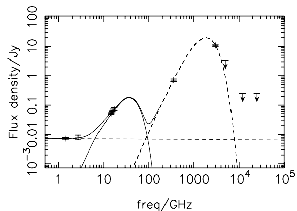
Figure 17. SED of L1111. uv sampled data points are shown at 1.4 and 2.7 GHz from the CGPS and Effelsberg 100 m. Data at 13.8 to 17.6 GHz from AMI are also shown. As are points at 850 \mu m (353 GHz) from Visser et al. (2001, 2003); and at 100, 60, 25 and 12 \mu m from the IRAS point source rejects catalogue. A power law is fitted to the data at 1.4 and 2.7 GHz which is shown as a dashed line. A modified greybody spectrum with \beta = 1.5 is fitted to the 850 and 100 \mu m data as described in the text and a MC spinning dust model from DL98 is fitted to the AMI data points, see text for details. The combined SED across the AMI band is shown as a solid line.
