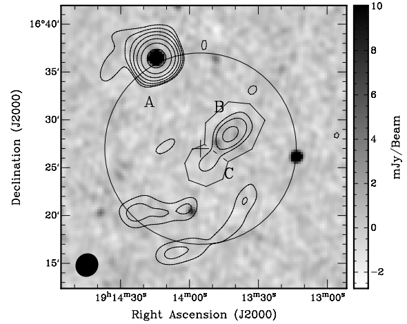
Figure 4. L709: CLEANED AMI combined channel data at 16 GHz are shown as contours with the levels as in Fig. 1. NVSS data at 1.4 GHz are shown in grey-scale and are saturated at 10 mJy peak to emphasize the structure in the map. The AMI pointing centre is indicated by a cross and the FWHM of the primary beam as a solid circle. The synthesized beam of AMI towards L709, 2.5 \times 2.4 arcmin 2 , is shown in the bottom left-hand corner as a filled ellipse. This map is not primary beam corrected. Example apertures are shown to indicate the division between sources ‘B’ and ‘C’ for flux extraction.
