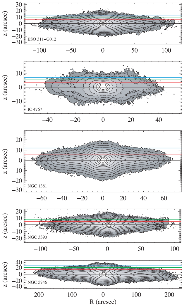
Figure 2. K -band images of the sample galaxies with the slits overlaid. Contours are separated by 0.5 mag. Images are taken from Bureau et al. (2006).
