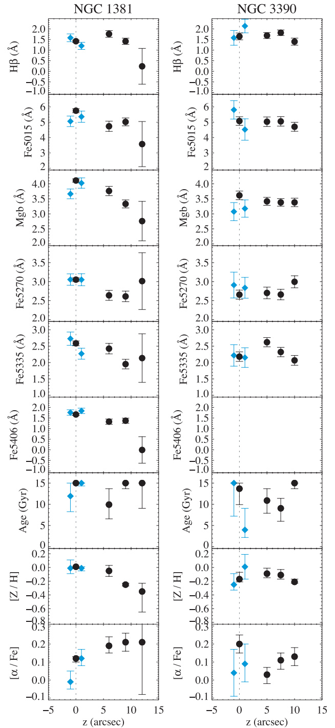
Figure 5. Lick indices and luminosity-weighted SSP-equivalent ages, metallicities and [\alpha/Fe] ratios as a function of the perpendicular distance to the major axis for NGC 1381 and 3390. Measurements are made at the centre of the galaxy (black circle at z = 0 ), two disc bins along the major axis (blue diamonds) and three points at increasing distance along the minor axis (black circles at z \neq 0 ). The disc bins correspond to spectra at z = 0 , but we added a spatial offset of \pm 1 arcsec for clarity in these plots. The z = 12 arcsec bulge spectrum in NGC 1381 has some line strengths that are consistent with an equivalent width of zero, and the uncertainties in [\alpha/Fe] for this bin extend over the full model grid. The position is shown merely for completeness. The Fe5406 feature is redshifted beyond the observed wavelength range for NGC 3390 and could therefore not be measured.
