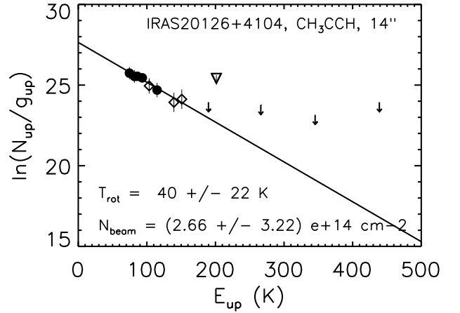
Fig. B.13. RTD fits for \text{CH}_3\text{CCH} .
