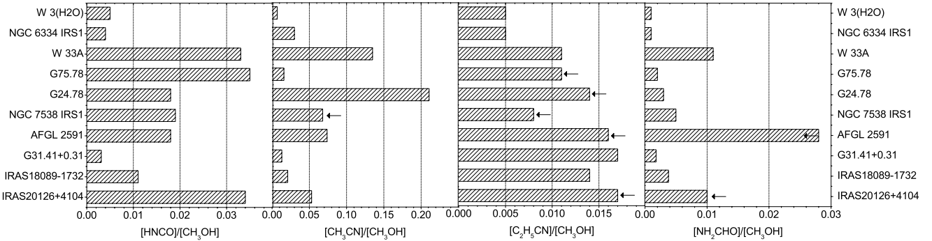
Fig. 11. Abundance ratios of N-bearing species \text{HNCO} , \text{CH}_3\text{CN} , \text{C}_2\text{H}_5\text{CN} and \text{NH}_2\text{CHO} with respect to \text{CH}_3\text{OH} (from RTD analysis). Arrows indicate upper limits.
