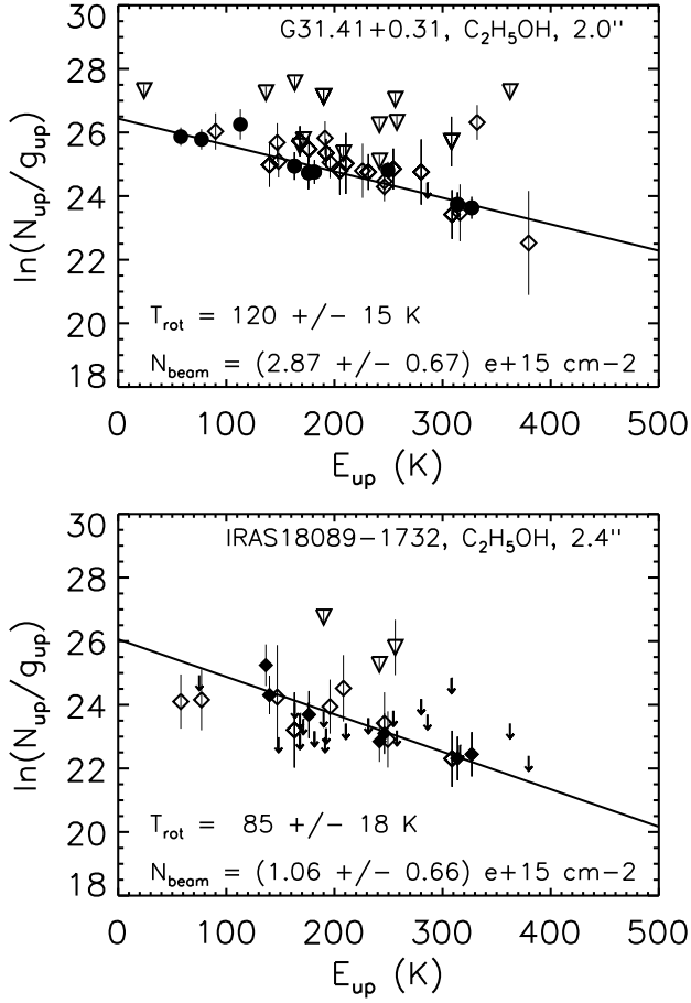
Fig. B.3. RTD fits for \text{C}_2\text{H}_5\text{OH} . No \text{C}_2\text{H}_5\text{OH} was detected in IRAS 20126+4104. For IRAS 18089 lines with S/N \gtrsim 1 have been used.
