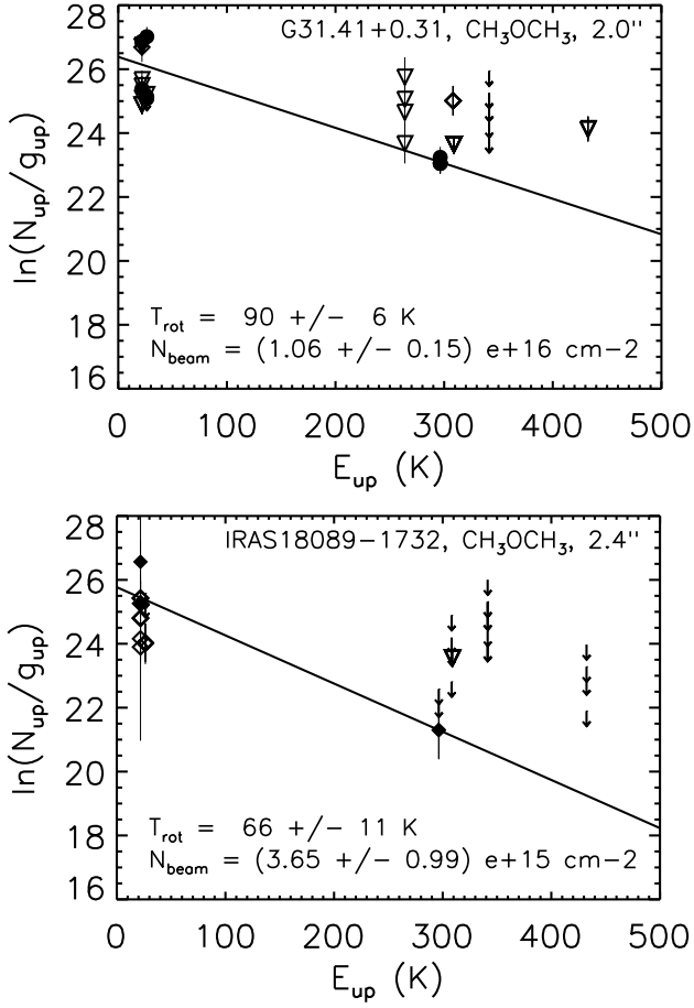
Fig. B.9. RTD fits for \text{CH}_3\text{OCH}_3 . No \text{CH}_3\text{OCH}_3 was detected in IRAS 20126+4104.
