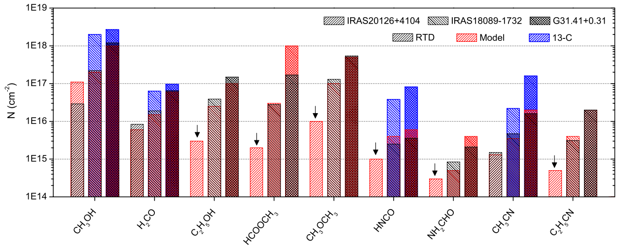
Fig. 5. Source-averaged column densities for the targeted warm species in \theta_{\text{T}}=100 K volume. Column densities from the RTD analysis are marked in black bars. The red and blue bars show column densities from the Weeds or CASSIS (CH 3 OH) models and from 13 C-isotopologue, respectively. Arrows indicate upper limits.
