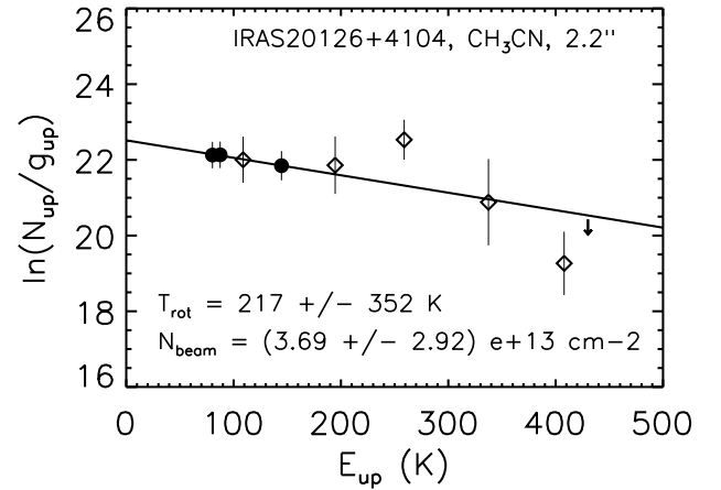
Fig. B.6. RTD fits for \text{CH}_3\text{CN} .
