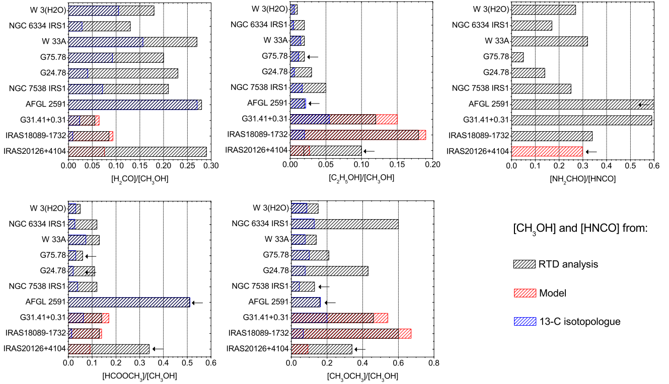
Fig. 10. Abundance ratios of complex species with respect to \text{CH}_3\text{OH} for oxygen-bearing species and \text{HNCO} for nitrogen-bearing species. The black bars indicate abundance ratios calculated with the \text{CH}_3\text{OH} and \text{HNCO} column density derived from the RTD analysis similar to BIS07. The red and blue bars indicate abundance ratios where \text{CH}_3\text{OH} and \text{HNCO} column densities are derived from CASSIS or Weeds (HNCO) model, respectively. Upper limits are marked with arrows.
