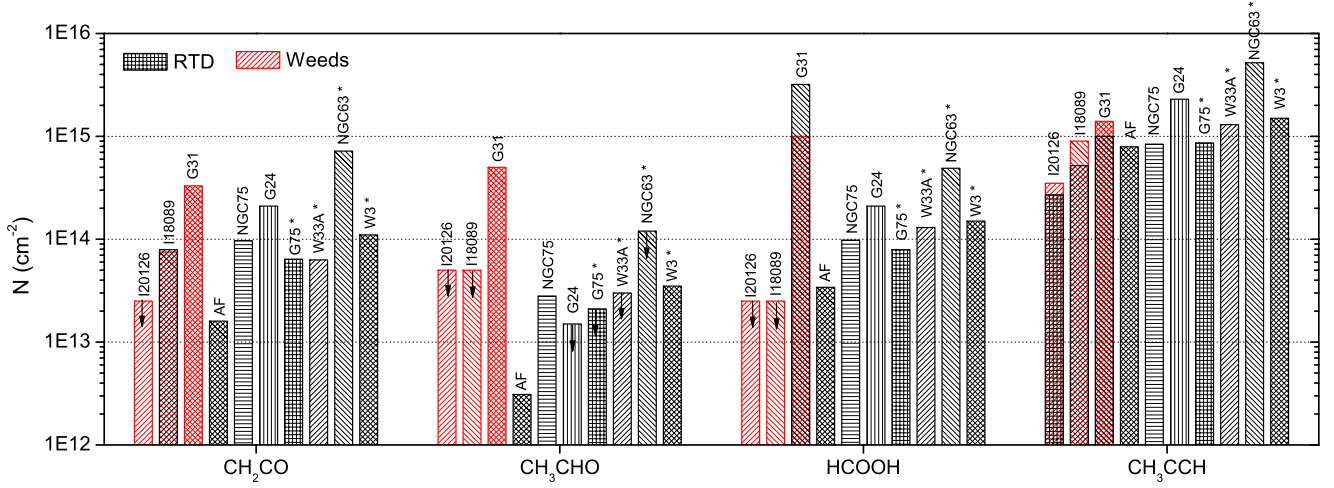
Fig. 9. Beam-averaged column densities for cold molecules in sources observed in this study and those from BIS07. Sources without disk structure are marked with an asterisk. Column densities from the RTD analysis are marked in black bars while the red bars show column densities from the Weeds model. Upper limits are indicated with arrows.
