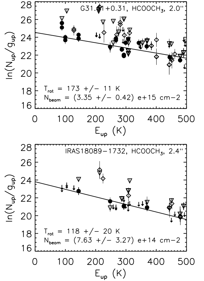
Fig. B.8. RTD fits for \text{HCOOCH}_3 . No \text{HCOOCH}_3 was detected in IRAS 20126+4104.
