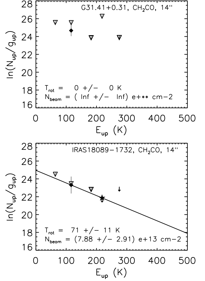
Fig. B.10. RTD fits for \text{CH}_2\text{CO} . No \text{CH}_2\text{CO} was detected in IRAS 20126+4104.
