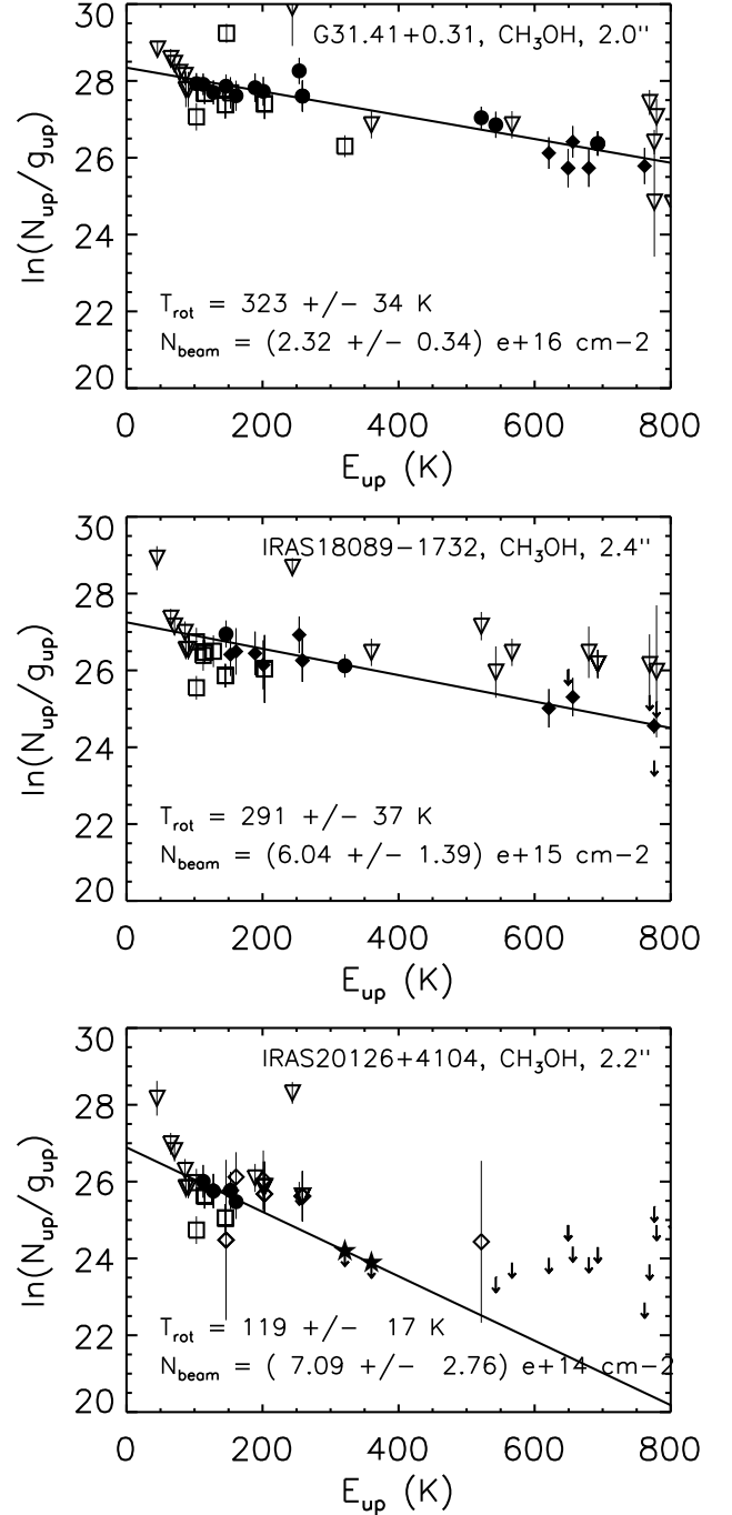
Fig. B.2. RTD fits for \text{CH}_3\text{OH} . Lines with E_{\text{up}} < 100 K are considered contaminated with the cold \text{CH}_3\text{OH} . Lines with S/N \gtrsim 1 are included in the fit.
