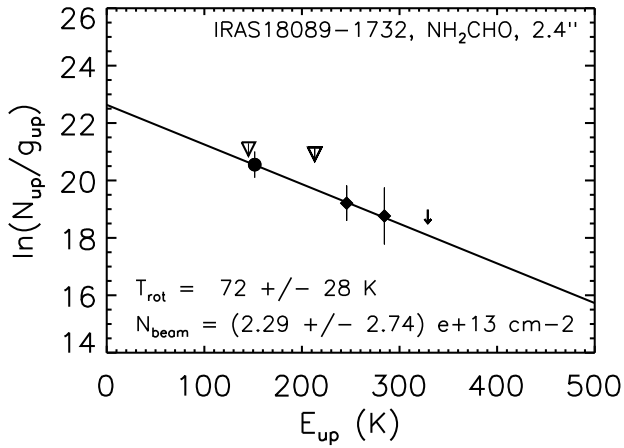
Fig. B.5. RTD fits for \text{NH}_2\text{CHO} . No \text{NH}_2\text{CHO} was detected in IRAS 20126+4104.
