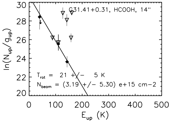
Fig. B.12. RTD fits for \text{HCOOH} .
