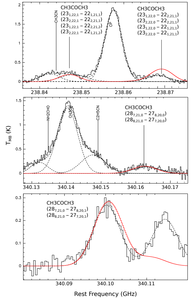
Fig. D.1. Beam-averaged spectra of CH 3 COCH 3 ( 23_{1/2,22,1}-22_{1/2,21,1} ), ( 23_{1/2,22,0}-22_{1/2,21,1} ), ( 28_{7/8,21,0}-27_{8/7,20,0} ) and ( 28_{7/8,21,0}-27_{8/7,20,1} ) towards G31.41+0.31 hot core. Dashed lines indicate Gaussian fits to the lines and red solid line show the Weeds model on the CH 3 COCH 3 lines at 100 K.
