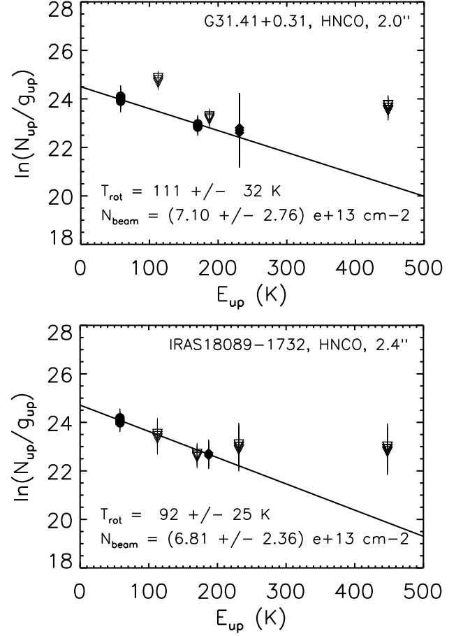
Fig. B.4. RTD fits for \text{HNCO} . No \text{HNCO} was detected in IRAS 20126+4104.
