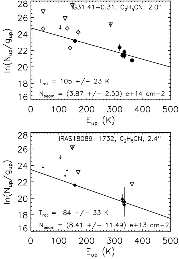
Fig. B.7. RTD fits for \text{C}_2\text{H}_5\text{CN} . No \text{C}_2\text{H}_5\text{CN} was detected in IRAS 20126+4104. For IRAS 18089 lines with S/N \lesssim 2 have been included in the fit.
