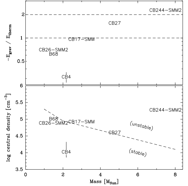
Fig. 6. Stability of starless cores. Top : ratio of gravitational potential to thermal kinetic energy vs. total gas mass ( 1.36 \times M_{\text{H}} ), both integrated within the N_2 column density contours (Table 5). The lower dashed horizontal line marks the bounding limit of -E_{\text{grav}}/E_{\text{therm}} = 1 , while the upper line marks the state of virialization at -E_{\text{grav}}/E_{\text{therm}} = 2 . Bottom : estimated central density (see Sect. 5.5) vs. total gas mass for the same starless cores. The dashed line marks the maximum stable density of a pressure-supported, self-gravitating modified (nonisothermal) BES (with photoelectric heating at the core boundary taken into account) as calculated by Keto & Caselli (2008, their Fig. 14). Typical estimated uncertainties on the source parameters are indicated as Y error bars on CB 4. The uncertainty in mass corresponds to the size of the label.
