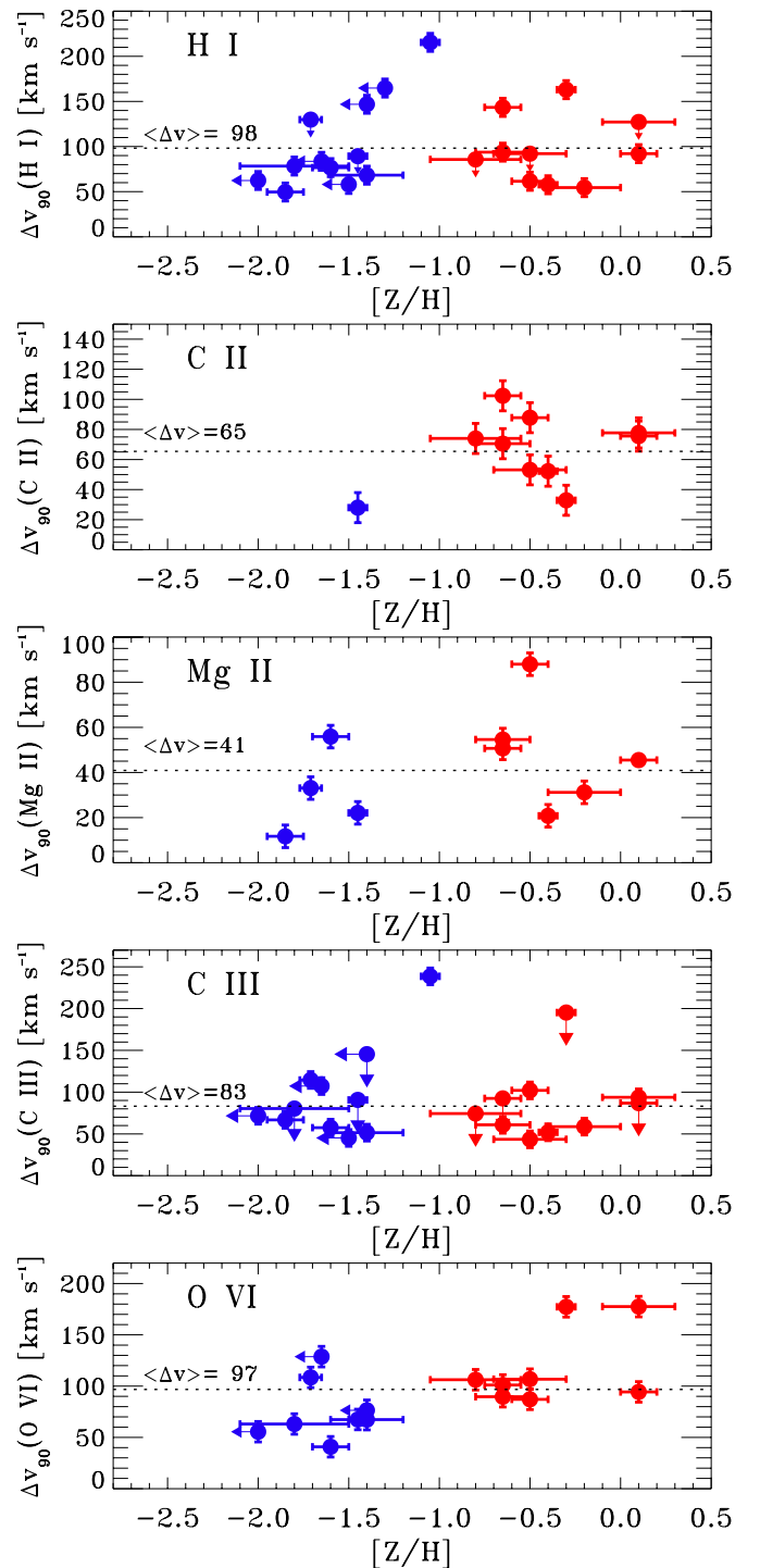
Figure 3. Comparison of velocity width \Delta v_{90} with metallicity for H I, C II, Mg II, C III, and O VI. Blue points indicate low-metallicity LLSs, and red points indicate high-metallicity LLSs. We use Si III as a proxy for C III in eight cases where it gives a better indication of the intermediate-ion kinematics. Saturated lines give upper limits on \Delta v_{90} . The z = 0.927 LLS toward PG 1206+459 is omitted from this plot; it shows a large velocity spread, covering \approx 600 \text{ km s}^{-1} . The sample size varies between ions since \Delta v_{90} can only be measured if the line is detected. C II is only detected in one of the metal-poor LLSs. In each panel the mean velocity width is annotated and shown with a dotted horizontal line. Note that each panel has a different scale on the y-axis.
