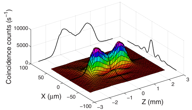
FIG. 3. (Color online) Measured coincidence rate R_{cc}(\mathbf{p}_-, z) \propto |V_{\text{project}}(\mathbf{p}_-, z)|^2 at a phase mismatch \varphi = -5.2 \pm 0.1 . The intersections with the \mathbf{p}_- = \mathbf{0} and z=0 planes are projected on the back and lateral sides of the plot.
