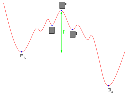
FIG. 2. A nucleation path from \Xi_\Lambda to \boxplus_\Lambda for Glauber dynamics. \Gamma in (1.10) is the minimal energy barrier the path has to overcome under the local variant of the Hamiltonian in (1.1).
