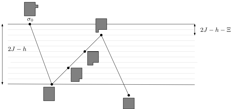
FIG. 9. Visualization of (3.18).
