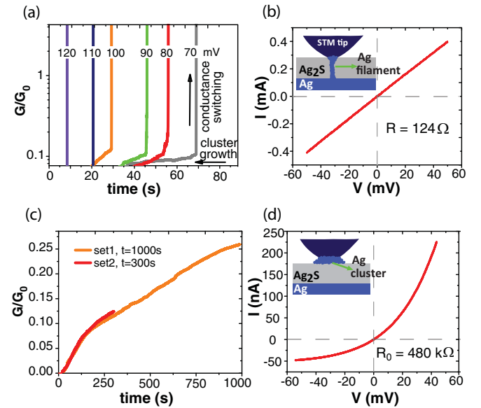
FIG. 4. (Color online) (a) Conductance switching induced at bias voltages \geq 70 mV. The plot shows the increase of the conductance above 1G_0 and a systematic decrease in the induction time with bias. (b) IV curve measured in the high-conductance state of the sample, indicating metallic behavior. (c) Conductance trace measured for 1000 s, applying a bias voltage of +50 mV. The trace in red presents another trace measured at +50 mV for 300 s. The trace does not show a sudden increase of the conductance for full switching. (d) IV curve measured at t = 60 s of a trace measured with +50 mV, demonstrating semiconducting behavior dominated by the bias-induced changes in ion concentration in the \text{Ag}_2\text{S} film (Ref. 12).
