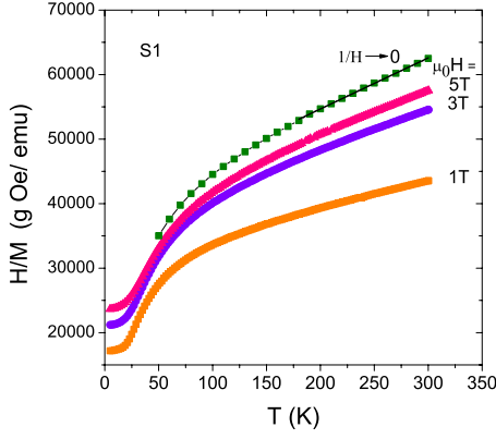
FIG. 4. (Color online) Inverse magnetic susceptibility H/M(T) of sample S1 for different external magnetic fields and extrapolated values 1/H \rightarrow 0 , according to the Honda-Owen method. Line represents the Curie-Weiss fit.
