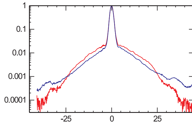
Figure 5. Cross-sections along the central horizontal SP beams (red curve) and along the forks (blue curve), for illumination with a laser beam of width 1.6 \mu\text{m} at a wavelength of 807 \text{ nm} .
