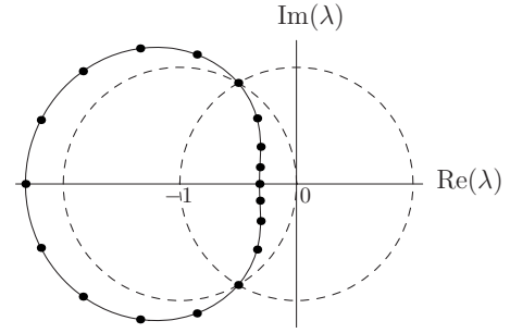
FIG. 11. Plot of the solutions of the characteristic equations [Eqs. (B4) and (B5)] for n=5 , m=11 , and k=0 . The dots are the roots, the solid curve is the contour described by Eq. (B4), and the dashed circles are unit circles with centers at 0 and -1 .
