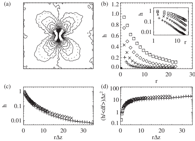
FIG. 3. (a) Shear stress \sigma_{xy} for point loading in the center and p = 10^{-3} . The response is coarse grained over a grain diameter [18] and averaged over 216 realizations (solid) and fitted to linear elasticity (dashed). (b)–(d) Spatial decay of the force fluctuations h . Squares, diamonds, crosses, and plus signs represent increasing pressures, ranging from p = 4.6 \times 10^{-5} to p = 3.2 \times 10^{-2} , respectively. (b) h as function of r . (c) Scaling collapse when h is plotted as function of r\Delta z . (d) Scaling collapse of relative fluctuations.
