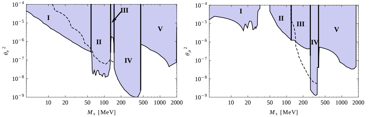
Figure 6: Direct accelerator bounds on the mixing angles. Left panel: \vartheta_e^2 bounds, taken from [37] (region I), [45] (region II), [40] (region III), [35, 55] (region IV) and [39] (region V). Right panel: \vartheta_\mu^2 bounds, taken from [42–44] (region I), [40] (region II), [41] (region III), [35] (region IV) and [38] (region V). The shaded regions are ruled out by the experimental findings. Dashed curves indicate mixing angle bounds given by original interpretation of PS191 experiment, but we do not use them to derive our final results, as explained in Sec. 4.3. The bounds are shown for the Majorana neutrino and are therefore two times stronger (see Section 4.4), while in the original works [34, 35] a single Dirac neutrino has been considered.
