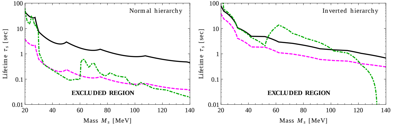
Figure 2: The lower bounds on the lifetime of sterile neutrinos, responsible for the mixings between active neutrinos of different flavours in the see-saw models (4). The bounds are based on the combination of negative results of direct experimental searches [34, 35, 37, 40–45] with the neutrino oscillation data [3]. The neutrino oscillation parameters are allowed to vary within their 3\sigma confidence intervals to minimize the lifetime. The solid black curve is based on our reinterpretation of PS191 data only , that takes into account charged and neutral current contributions (see Sec. 4.3). The interpretation of the PS191 experiment, taking into account only CC interactions (used e.g. in the previous works [12, 17]) is shown in magenta dashed line. The bound from peak searches experiments only [37, 40–45] is plotted in green dot-dashed line.
