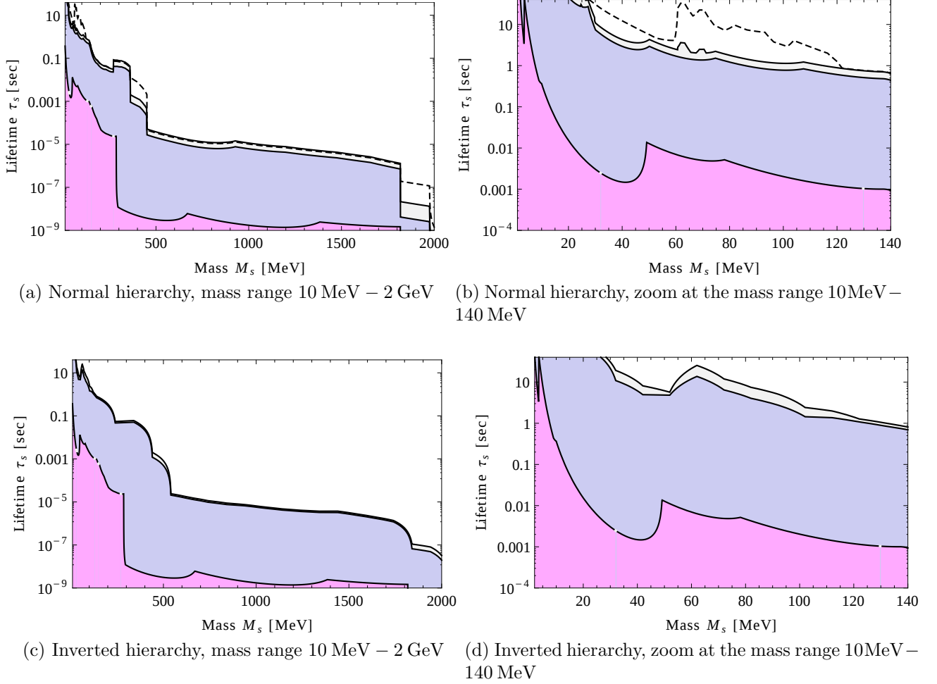
Figure 7: The resulting lower bounds on sterile neutrino lifetime \tau_s as a function of their mass, obtained by requiring that two Majorana sterile neutrinos are responsible for neutrino oscillations and their parameters do not contradict the negative results of direct experimental searches. In all figures the upper curve comes from using of the best fit neutrino oscillation parameters, the middle one – from their variation within the 3\sigma limits, and the lower one does not take into account neutrino oscillation data and puts all three mixing angles equal to their direct experimental bounds. The dashed line for NH corresponds to the best-fit values of PMNS parameters with \theta_{13} = 0 and shows how much the bounds on the lifetime relax for non-zero value of \theta_{13} (see text, Section 5 for discussion).
