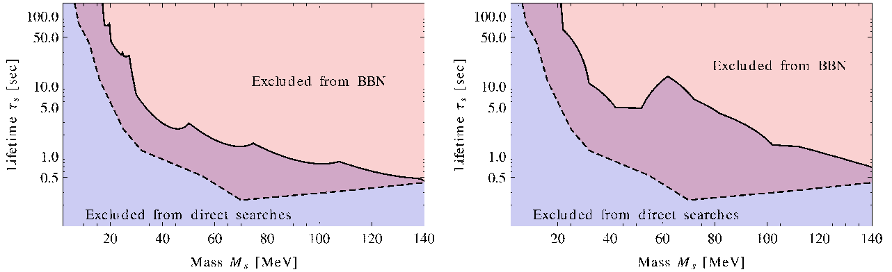
Figure 8: Experimental lower bounds on the lifetime of sterile neutrinos (solid line), combined with the upper bounds coming from the BBN (dashed line) [22]. Left panel: normal hierarchy, right panel: inverted hierarchy. Shown are 3\sigma lower bounds from the Fig. 7 and the weakest bound from primordial nucleosynthesis (based on the CMB measurements of primordial Helium abundance, yielding Y_p = 0.445 at the 3\sigma level [6, 61], see text for details).
