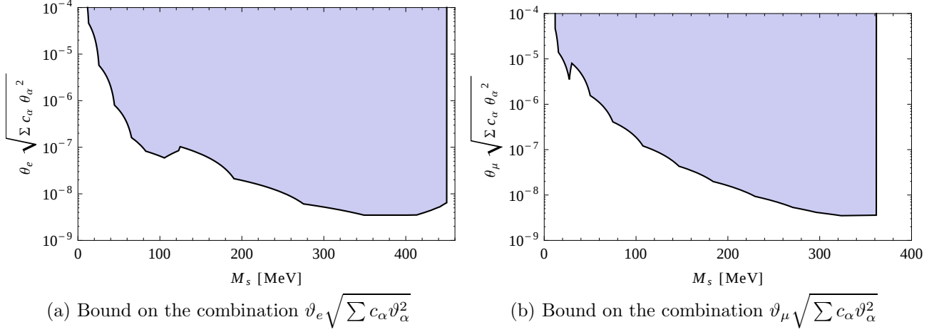
Figure 5: Direct accelerator bounds on the combination of active-sterile neutrino mixing angles, resulting from the reanalysis of the PS191 experiment [34, 35], taking into account decays of sterile neutrino through both charged and neutral currents and their Majorana nature. The shaded region is excluded. The case, analyzed in the original works [34, 35] (decay of sterile neutrino through the charged current only) corresponds to the choice c_e = 1 , c_\mu = c_\tau = 0 , for details, see Sec. 4.3. We plot the bounds for two Majorana neutrinos (as in Fig. 6) while in the original works [34, 35] a single Dirac neutrino was analyzed.
