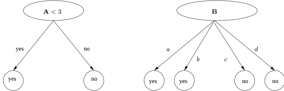
Figure 3.1: The two possible decision tree for Example 3.2.1 based on the gain criterion.
