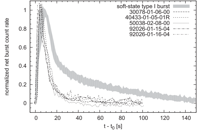
Figure 12. Light curves of five type I bursts in the hard state plotted against the average profile of the 22 single-peaked type I bursts featuring the longest and brightest decays (see B14), all of which are instead observed in the soft state. The net bursts counts have been normalized so that the average flux during the burst peak (which is defined as the interval during which the flux is above 90 per cent of the burst peak flux) is 1. The vertical extent of the shaded region indicates the standard deviation of the soft-state sample. The hard-state type I bursts were randomly chosen among those taking place on top of a stable persistent emission, i.e. outside humps, and showing no overlapping type II bursts during the first 40 s of the type I burst.
