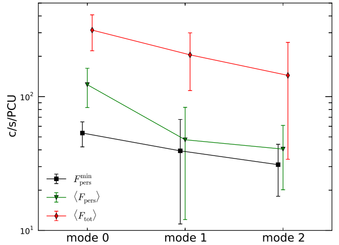
Figure 4. The average values of F_{\text{pers}}^{\text{min}} , \langle F_{\text{pers}} \rangle and \langle F_{\text{tot}} \rangle during mode-0, -1 and -2 type bursts (see Section 4.1). The error bar indicates the standard deviation in each sample.
