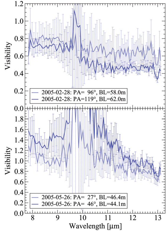
Fig. 3. Spectrum of the visibility F_{\text{corr}}/F_{\text{tot}} between 8 and 13 \mu\text{m} as observed on February 28 ( top panel ) and on May 26, 2005 ( bottom panel ). Wavelengths 9.5 < \lambda < 10.1 \mu\text{m} are strongly affected by the atmospheric ozone band. Errors are dominated by the (systematic) errors in F_{\text{tot}} .
