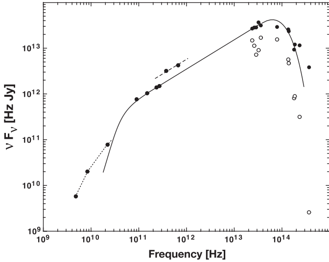
Fig. 6. Overall spectrum of the core of Centaurus A. Open circles show observed flux values, filled dots are corrected for the foreground extinction of A_V = 14 mag (compare Fig. 5). The synchrotron spectrum (solid line) shows an optically thin power-law F_\nu \sim \nu^{-0.36} which cuts off exponentially at \nu_c = 8 \times 10^{13} Hz, and is self-absorbed below \nu_1 \approx 4.5 \times 10^{10} Hz. Evidence for variability exists around 3 \times 10^{11} Hz (dashed line through photometry in 1991) and above \nu_c (various epochs between 1997 and 2005, cf. Table 2). The excess at cm wavelengths ( \nu < 2 \times 10^{10} Hz, connected by dotted lines) is due to optical thick components of larger size.
