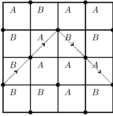
Fig. 3. \Pi sampling \Omega . The dashed lines with arrows indicate the steps of \Pi .
