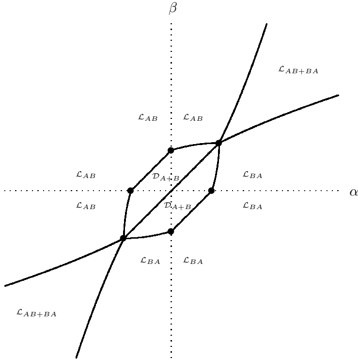
Fig. 10. Full phase diagram for 1 - p_c < p < p_c .
