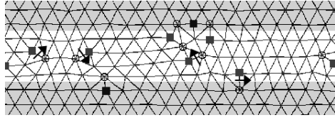
Figure 21. Triangulation of the static ground state structure for w/b_0 = 3.48 and \Delta = 0.05 . The arrows indicate the Burgers vectors of the dislocations. Shown is a characteristic segment of the total channel length L = 500a_0 .
