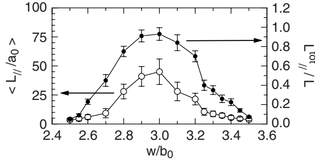
Figure 24. The ‘correlation’ length \langle L_{\parallel} \rangle (○) and the fraction L_{\parallel}^{tot}/L (●) of regions with n = 3 rows versus w/b_0 .
