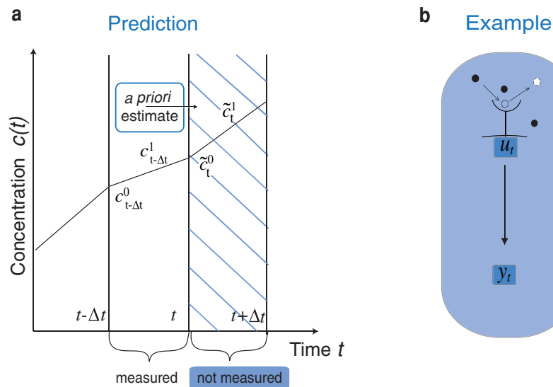
Figure 2 | Iterative prediction scheme for receptor sensing with memory. (a) At each time step the concentration profile is measured and updated (see also green and orange equation boxes in Fig. 1). Receptor sensing is based only on past measurements to make an a priori estimate (prediction) for both concentration \tilde{c}_t^0 and slope \tilde{c}_t^1 with accuracy limited by the Cramér-Rao bound. (b) Simplest implementation of the scheme in a cell-signalling network. Upon binding and unbinding of external ligand, the receptor activity u(t) induces production of molecule species y . For slow reaction rate, the production of y mirrors the input with a delay, reproducing the condition of the prediction scheme in which the current time measurement is not accessible. For details see sections S4A and S5A in SI.
