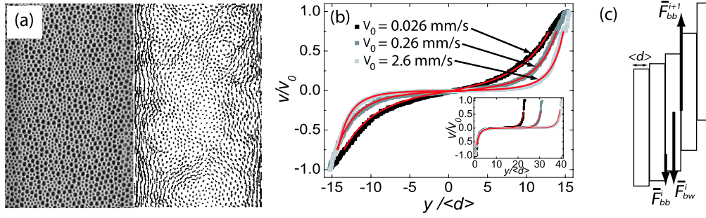
FIG. 2 (color online). (a) Experimental image of bidisperse foam (left) and corresponding bubble tracks (right). Note the swirling motion. (b) Rescaled velocity profiles v/v_0 for W = 7 cm and v_0 as indicated, compared to profiles obtained from our model Eq. (5) with \alpha = 2/3 , \beta = 0.36 , and k = 3.75 [thin solid (red) lines]. Inset: v/v_0 for v_0 = 8.3 mm/s and W equal to 5, 7, and 9 cm—for convenience, we chose the origin at the left boundary here. (c) Illustration of the model defined by Eq. (5).
