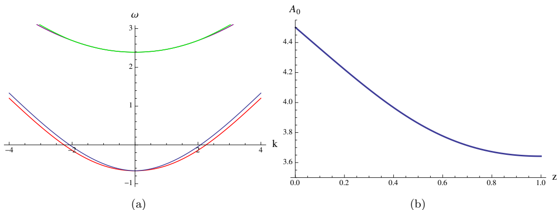
Figure 2. (a): Fermionic spectrum in the self-consistent solution of the fermion+gauge field system at q\mu = 4.5 , z_w = 1 and m_\Psi = 1 . The red and blue curves represent the modes with positive and negative eigenvalues of \hat{k}_i \Gamma^i \Gamma^0 respectively. (b): The profile of the gauge field sourced by the fermions.
