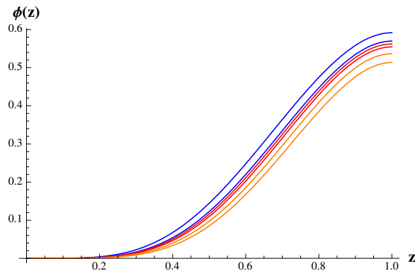
Figure 9. Profiles of the bulk scalar wavefunction \phi(z) for \Delta_\phi = 4.6765 , \Delta_\phi = 4.8541 (two blue curves), \Delta_\phi = 4.9438 , \Delta_\phi = 5.0341 (two red curves, - proximity of the critical point), \Delta_\phi = 5.379 , and \Delta_\phi = 5.4925 (two orange curves). Crossing the critical point \Delta_\phi = 2\Delta_\Psi = 5 does not lead to any singularities in the bulk wavefunction. The other parameters here are \eta_5 = 1 , \mu q = 4.5 , z_w = 1 , q_\phi = 2 , \omega_D = 0.7 .
