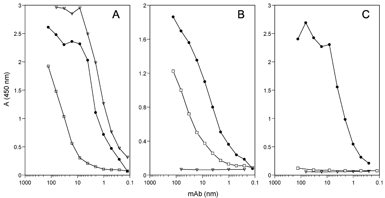
Fig. 1. Binding of mAbs E2, E3 and E8 to human, bovine and porcine lactoferrin. Polysorp plates were coated with 100 \mu\text{l} of 1 \mu\text{g/ml} hLF (A), bLF (B) or pLF (C) in PBS and incubated with serial dilutions of E2 (□), E8 (●) and E3 (▽). Bound mAb was detected by incubation with peroxidase labelled goat anti-mouse immunoglobulin. The A_{450} values of converted substrate are plotted against the amount of mAb added.
