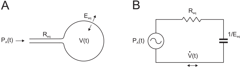
Figure 3.1: Simple compartment model fitted in single frequency FOT. A: Mechanical model of a single airway with resistance R_{eq} and elasticity E_{eq} . B: Equivalent electrical circuit.
