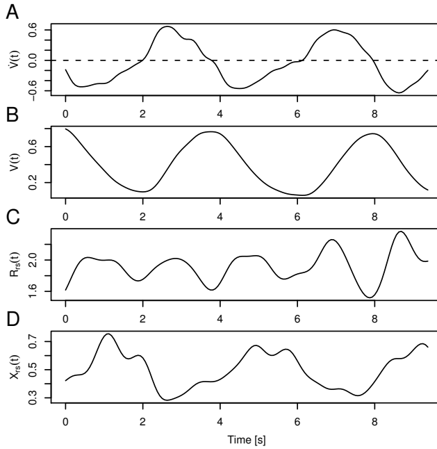
Figure 3.2: Typical forced oscillation signal from input impedance measurements in a healthy subject. A: Flow (positive: expiration, negative: inspiration). B: Volume. C: Estimated respiratory system resistance. D: Estimated respiratory system reactance.
