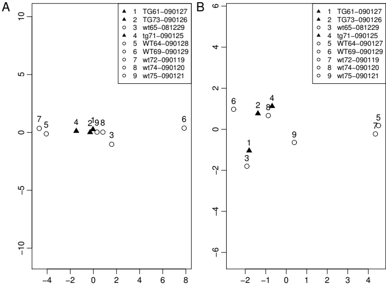
Figure 4.10: 2D MDS reconstruction of 1D Wasserstein distances. A: HC dataset (hippocampus). B: PAR dataset (total brain).
