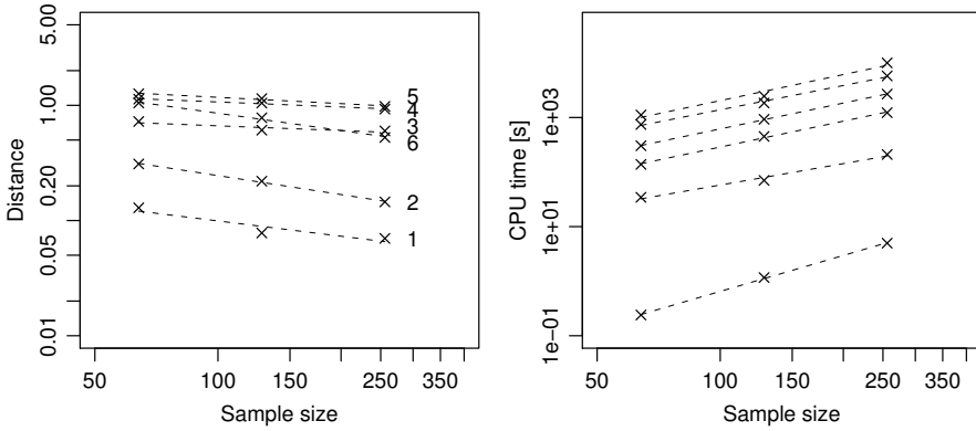
Figure 2.17: Dependence of estimated self-distances on sample size. Left panel: Generalized Wasserstein distances (with respect to rigid motions) for embedding dimensions 1 to 6. The embedding dimension has been indicated on the right side of the regression lines. Right panel: CPU time needed for these calculations, with a slope of roughly 3/2 (for dimensions greater than two).
