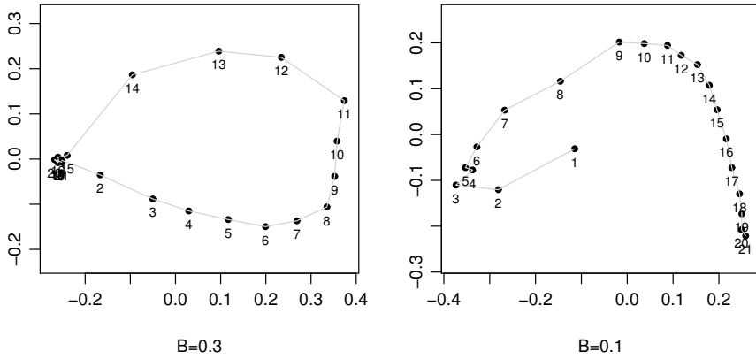
Figure 2.10: Two-dimensional MDS representation of Wasserstein distances for coupled Hénon systems. Coupling strength varied as in Figure 2.9. Left panel: Equal Hénon systems ( B = 0.3 ). Right panel: Distinct Hénon systems ( B = 0.1 ). The numbers next to the dots indicate the coupling strength, with larger number representing coupling strengths closer to 1.0. The points in the left panel constitute a closed curve, since the dynamics of strongly coupled equal Hénon systems is very similar to that of uncoupled equal Hénon systems. The points in the right panel show a different pattern, since the dynamical behavior of two distinct uncoupled Hénon systems is not similar, confer Fig. 2.9.
