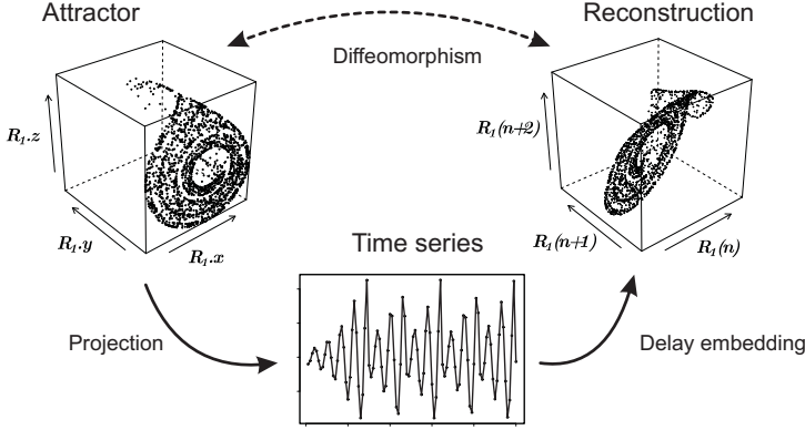
Figure 2.1: The methodology of attractor reconstruction via delay embeddings. The true attractor is projected into a time series by some measurement function, from which an image of the attractor can be formed by delay reconstruction, up to some diffeomorphism.
