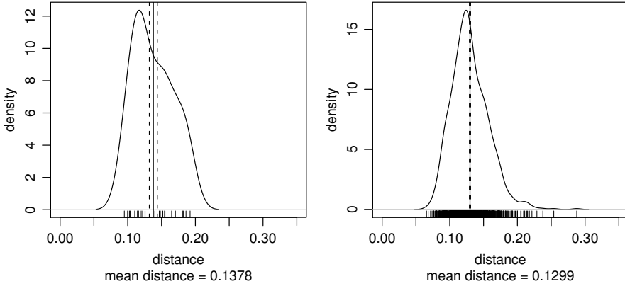
Figure 2.5: Distribution of Wasserstein self-distances under bootstrapping in the Hénon map, for 512 sample points. Left panel: N = 25 bootstraps. Right panel: N = 1000 bootstraps. Curves are kernel density estimates and the rugs at the bottom indicate the individual values of the distances. Vertical lines show mean distance (solid) and its standard deviation (stippled) over all N realizations.
