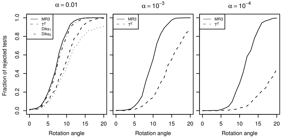
Figure 5.7: Estimated power functions for translated (10 standard deviations), then rotated diagonal Gaussians with unit variance against the scattered Fisher distribution (scaled by a unit Gaussian) as a function of relative rotation angle. Sample size N = 10 . Note the small power at angle zero.
