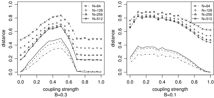
Figure 2.11: Distances for coupled Hénon systems for different bootstrap sizes. Coupling strength varied from C = 0.0 to C = 1.0 in steps of 0.05. Left panel: Equal Hénon systems ( B = 0.3 ). Right panel: Distinct Hénon systems ( B = 0.1 ).
