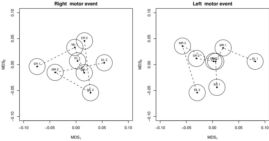
Figure 6.5: The MDS representation of the quadratic Wasserstein distances. E: EMG, M: Motor cortex, L: Left, R: Right, 1: 100 ms before motor event, 2: 250 ms after motor event. The components of the invariant eigenvectors are again given by the size of the surrounding circles; compare with Figure 6.4.
