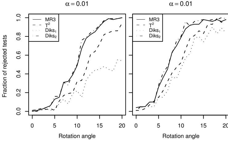
Figure 5.8: Adjusted estimated power functions. Left: translated (10 standard deviations), then rotated diagonal Gaussians with unit variances as a function of relative rotation angle. Right: translated (10 standard deviations) then rotated diagonal Gaussians with unit variance against the scattered Fisher distribution (scaled by a unit Gaussian) as a function of relative rotation angle. Sample size N = 10 . Results based on 100 realizations of 10^4 permutations each.
