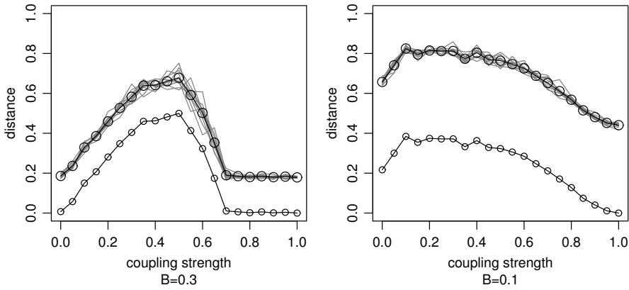
Figure 2.9: Distances for coupled Hénon systems (see text for details of the coupling). Coupling strength varied from C = 0.0 to C = 1.0 in steps of 0.05. Left panel: Equal Hénon systems ( B = 0.3 ). Right panel: Distinct Hénon systems ( B = 0.1 ). Top curves are uncorrected distances, the lower curves are corrected by subtracting the minimum distance encountered. Only the mean curve is depicted at the bottom.
