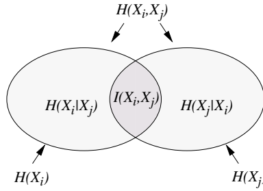
Figure 6.2: Relationship between mutual information and (conditional) entropies. More formally, one finds I(X_i, X_j) = H(X_i, X_j) - H(X_i|X_j) - H(X_j|X_i) = H(X_i) - H(X_i|X_j) = H(X_j) - H(X_j|X_i) ; after Cover and Thomas (1991).
