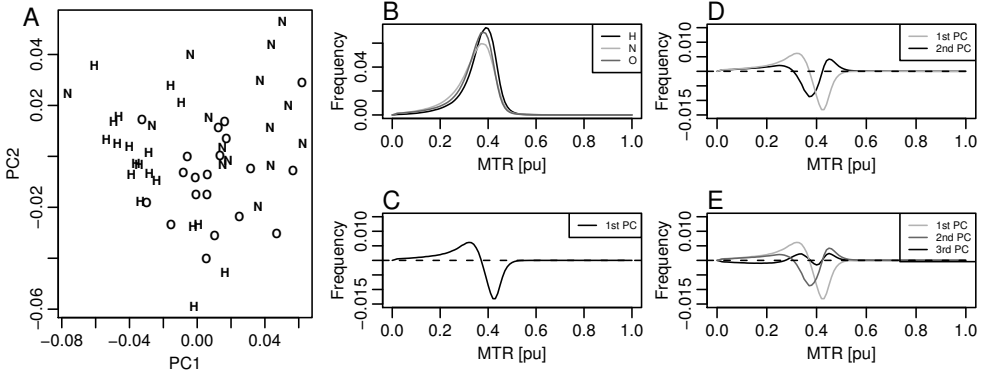
Figure 4.3: MDA/LDPCA of PAR dataset. A: Scores for first two principal components. B: Mean MTR histograms (100 bins). C: First principal component (64.4% of variance). D: First two second PCs (92.4% of variance). E: First three PCs (95.8% of variance).
