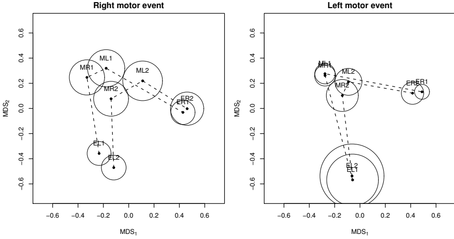
Figure 6.4: MDS results for the circular variances of Fig. 6.3; the four signals at two distinct time steps before and after the left/right motor events are presented as points (circle centers) in a two-dimensional functional space (Friston et al., 1996). The circles around the points indicate the invariant eigenvector for the uniformity (i.e., the radius of a circle is the value of the eigenvector’s corresponding component); recall the sketch of Page Ranking in Section 6.2.3. E: EMG, M: Motor cortex, L: Left, R: Right, 1: 100 ms before motor event, 2: 250 ms after motor event; see text for further details.
