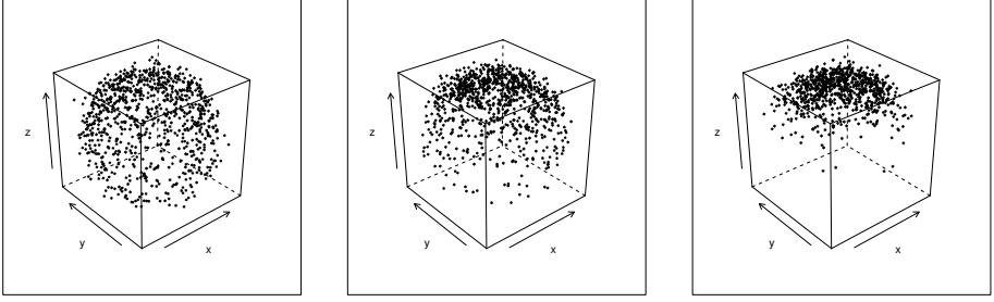
Figure 5.3: Scattered Fisher distribution, visualized by 1000 randomly drawn points in the unit-cube. Left: Concentration parameter \lambda = 1 . Middle: Concentration parameter \lambda = 2.5 . Right: Concentration parameter \lambda = 5 .
