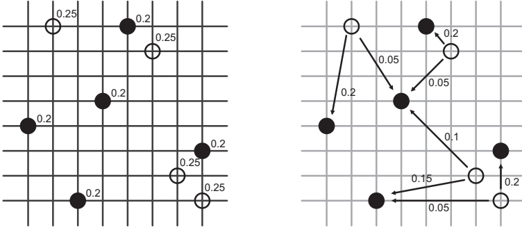
Figure 2.2: Example optimal transportation problem in the discrete case. Open circles correspond to the first measure, filled circles correspond to the second measure. For simplicity, the points are distributed on a grid with unit spacing. Left panel: Initial configuration. Numbers indicate probability mass at each point. Right panel: An optimal transportation plan with Wasserstein distance W \approx 3.122 . The numbers next to the arrows indicate how much probability mass is transported from the first measure to the second measure.
