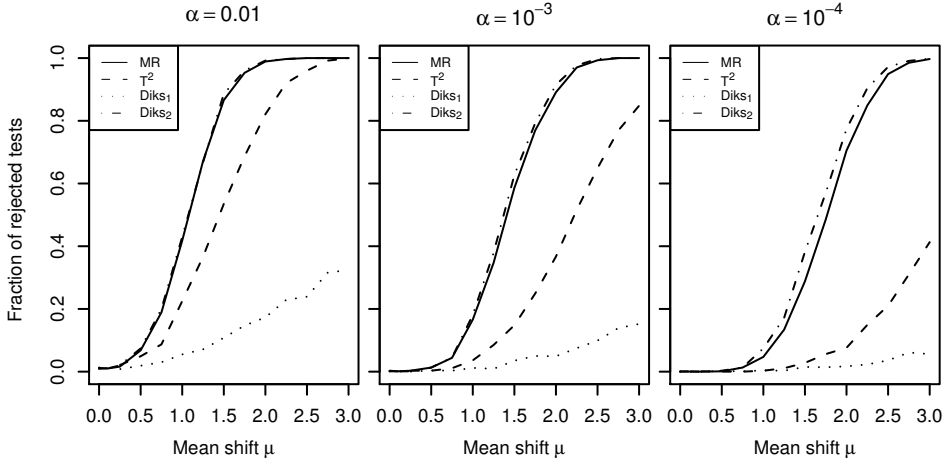
Figure 5.1: Estimated power functions for the family of Gaussian distributions with covariance matrix the identity and mean shifted a distance \mu away from zero. Sample size N = 10 .
