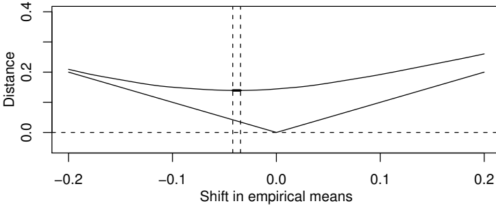
Figure 2.16: Translated Wasserstein distances for two normalized realizations ( n = 50 ) of a \mathcal{N}(0, 1) random variable. Lower solid curve: distance between empirical means against translation. Upper solid curve: Wasserstein distance W(\mu_\tau, \nu) . The minimum, attained in the indicated interval (dotted lines), is the Wasserstein distance with respect to translations, W^t(\mu, \nu) .
