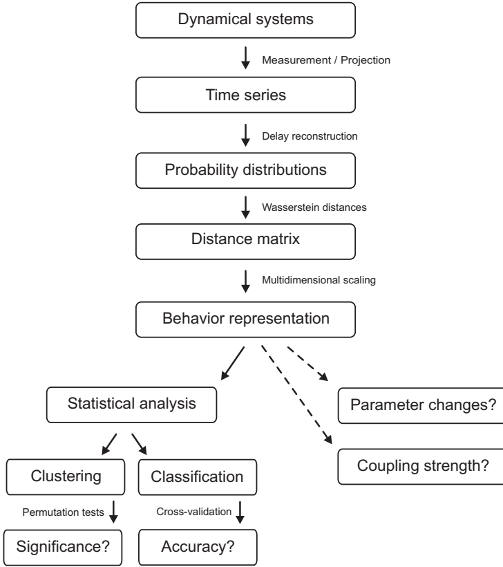
Figure 2.3: Outline of the methodology of distance-based analysis of dynamical systems and time series. The solid arrows indicate the main flow of steps. The broken arrows indicate optional steps that are applicable in particular situations. Note that we do not discuss clustering methods in this paper, as they are generally well-known.
