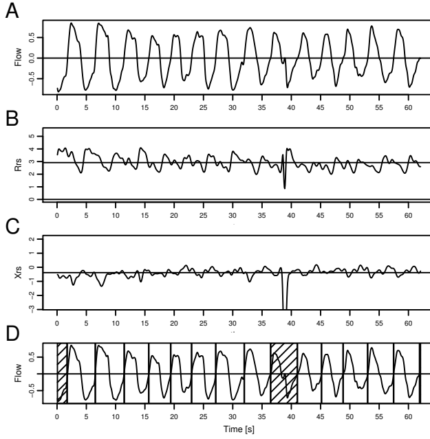
Figure 3.3: Artifact detection in respiratory impedance signals. A: Flow signal sampled at 16 Hz. B, C: Estimated respiratory resistance R_{rs} and reactance X_{rs} . Possible expiratory flow limitation is visible around T = 38s , resulting in large R_{rs}/X_{rs} values at minimal flow that lie outside the depicted confidence region (here: X_{rs} ). D: Flow signal after artifact detection and preprocessing. Distinct respiratory cycles are separated by zero-crossings of flow, and the shaded regions are rejected as incomplete or unreliable.
