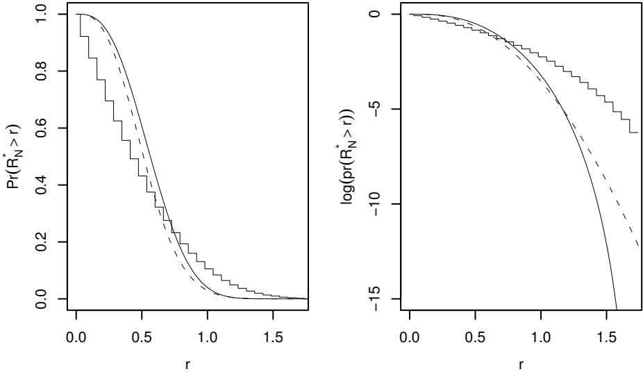
Figure 5.5: Comparison of significance probabilities for resultant lengths of spherically symmetric (smooth curve) and one-dimensional symmetric random walk (piecewise-linear curve) in three dimensions for N = 10 steps. Dotted curve shows the asymptotic case.
