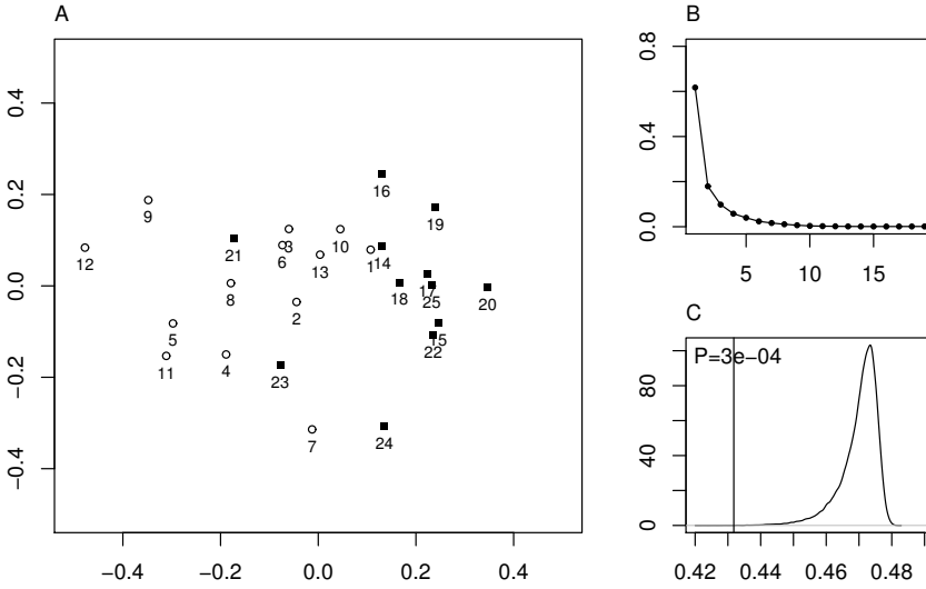
Figure 2.15: Results for Wasserstein distances W of normalized and centred data. Representation as in Fig. 2.14.
