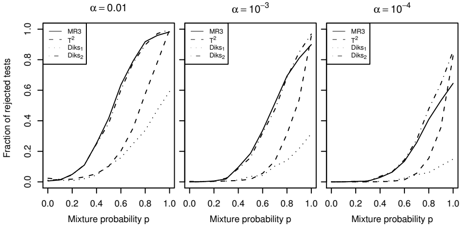
Figure 5.4: Estimated power functions for the mixture of the scattered Fisher distribution 2F3_5 with the uniform distribution on the sphere S^2 , varying the mixture probability p that a sample vector arises from the first distribution. Sample size N = 10 .
