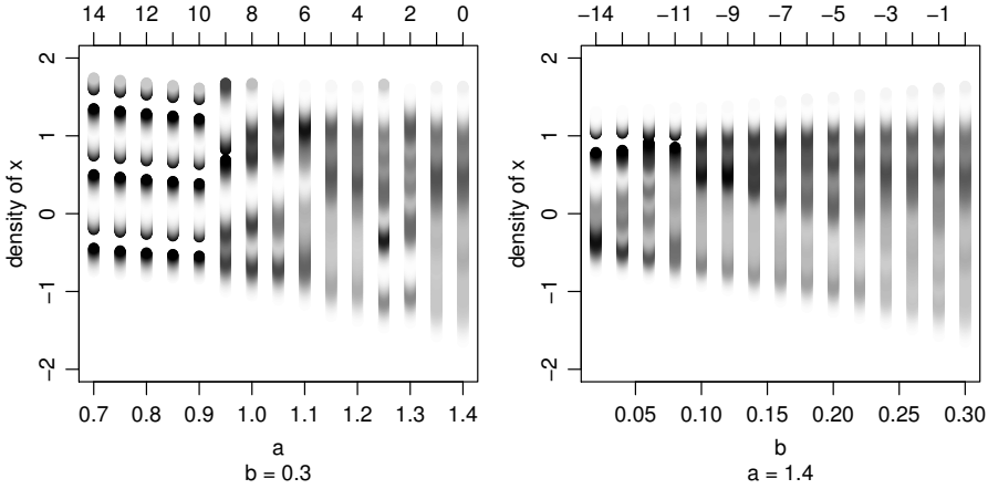
Figure 2.7: Invariant measures of the x -variable in the Hénon system, for different values of the parameters. Left panel: Variation in parameter a , with constant b = 0.3 . Right panel: Variation in parameter b , with constant a = 1.4 . See text for details of the parameter values used. Darker shade indicates large time averages, and lighter shade smaller time averages. Top axis of the panels shows indices of the dynamical systems used in Fig. 2.8.
