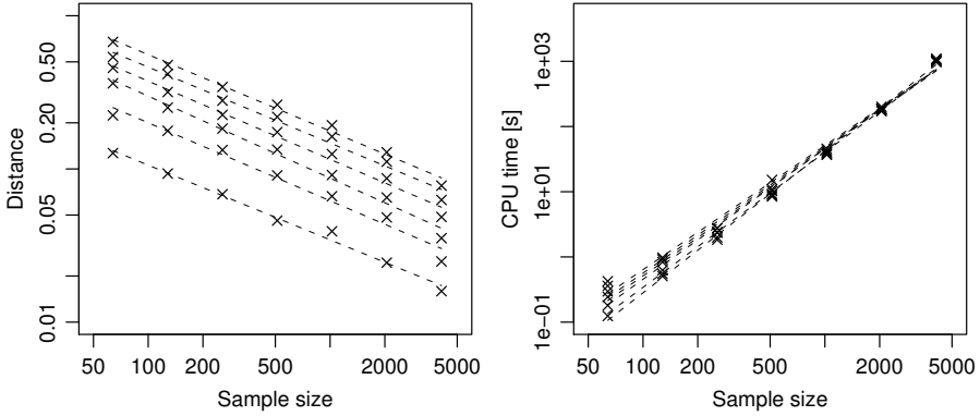
Figure 2.4: Dependence of Wasserstein self-distances on sample size. Left panel: Wasserstein distances for embedding dimensions 1 (lowest curve) to 6 (highest curve). The deviation from the true value of zero is an indication of the statistical error. The slope of the regression lines is roughly -1/2 , which is the typical scaling behavior of Gaussian noise. Right panel: CPU time needed for these calculations, with a slope of roughly 2, i.e., a quadratic dependence on sample size.
