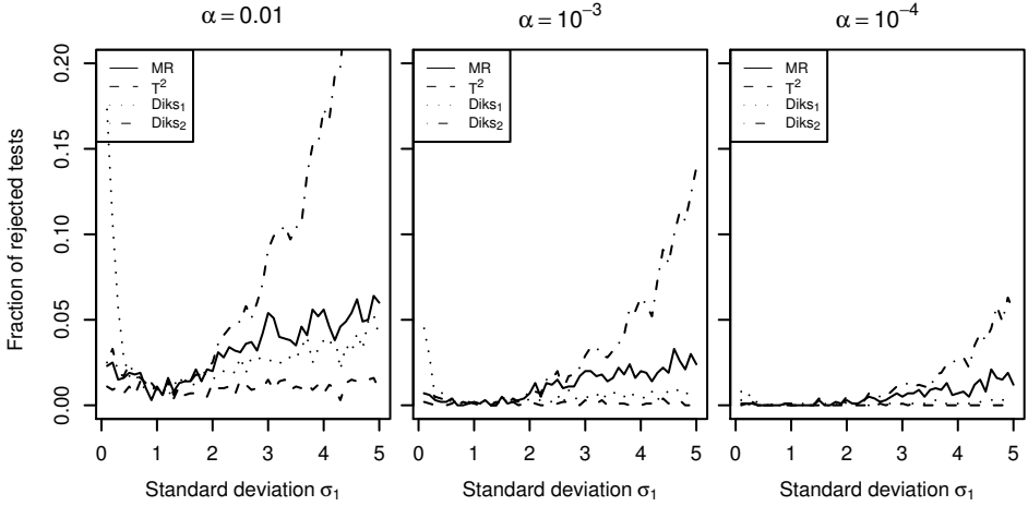
Figure 5.2: Estimated power functions for the family of Gaussian distributions, varying the standard deviation \sigma of a single axis. Sample size N = 10 . Note the small range of the power.
