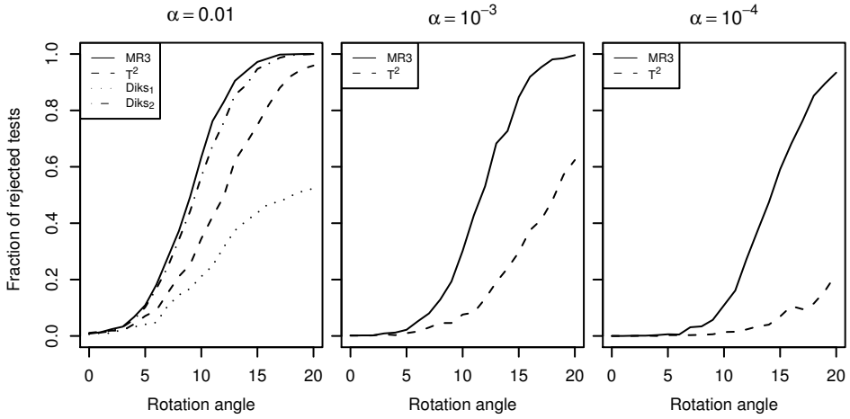
Figure 5.6: Estimated power for translated (10 standard deviations), then rotated diagonal Gaussians with unit variances as a function of relative rotation angle. Sample size N = 10 .
