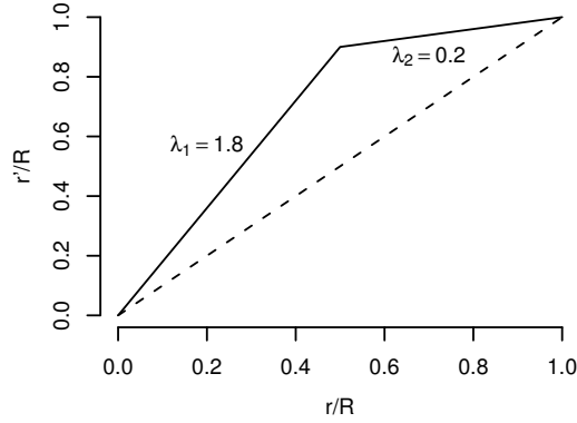
Figure 5.9: Generation of spherical deformations. The plot shows the behaviour of the deformation field in a one-dimensional projection along a radial direction. The volume at normalized distance r/R from the centerpoint of the sphere (radius R ) is mapped radially to r'/R . For r < R/2 the length of the deformation vectors expands linearly, r' = \lambda_1 r , attaining its maximum at half radius r = R/2 . For r > R/2 the length shrinks linearly by \lambda_2 = 2 - \lambda_1 , ensuring continuity at the boundary. The stippled line shows the case of no deformation ( \lambda_1 = 1 ).
