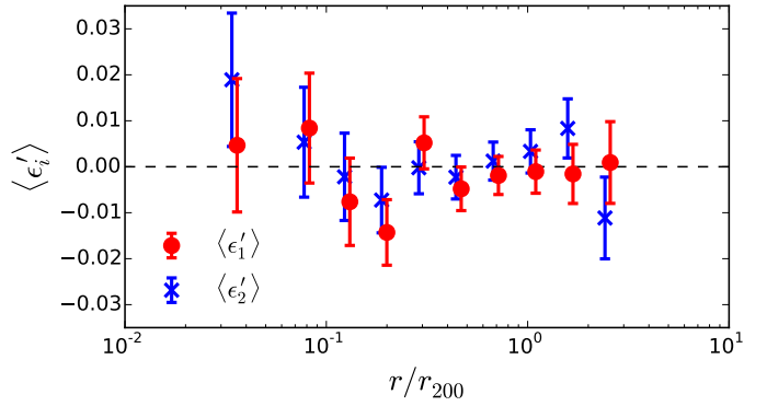
Figure 4.10: Mean ellipticity components of spectroscopic plus red sequence satellite galaxies in a frame rotated by the position angle of the BCG, probing the alignment of satellites with the cluster BCG. BCG position angles are measured with GALFIT, while the shapes of satellite galaxies are measured with KSB. Red circles show alignments with respect to the major ( \epsilon'_1 > 0 ) and minor ( \epsilon'_1 < 0 ) axes of the BCG, while blue crosses show alignments at 45^\circ rotations.
