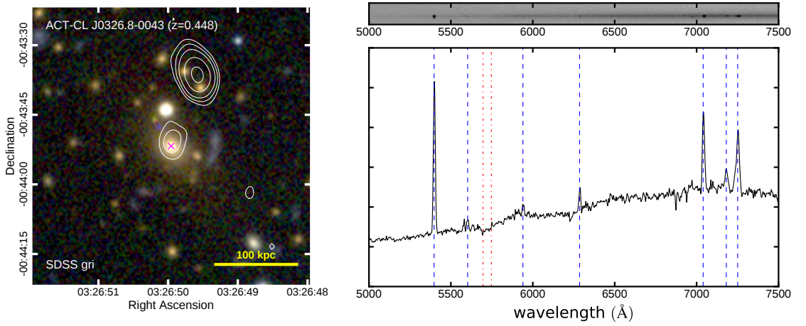
Figure 3.8: The BCG of ACT-CL J0326.8–0043 at z = 0.45 . Left: Optical gri image from SDSS with 1.4 GHz contours from the FIRST survey overlaid in white and shown at (3, 5, 8, 15, 25) \sigma levels, where \sigma = 0.14 \text{ mJy beam}^{-1} . The BCG is marked with a magenta cross and the thick yellow line in the bottom-right corner is 100 kpc wide, corresponding to 17''.4 at the cluster redshift. North is up and East is left. Right: Optical one- (bottom) and two-dimensional (top) Gemini/GMOS spectra. The former is smoothed with a 3-pixel boxcar. In the bottom panel, detected emission lines are marked with dashed blue lines (in order of increasing wavelength: [O II], Ne III, H \delta , H \gamma , H \beta and [O III] \lambda\lambda 4959, 5007 ); the Ca II K,H absorption doublet is marked with dash-dotted red lines. The asymmetric broadening of the [O III] \lambda 5007 line is an artifact introduced by interpolating the GMOS chip gaps. The vertical axis is in arbitrary units.
