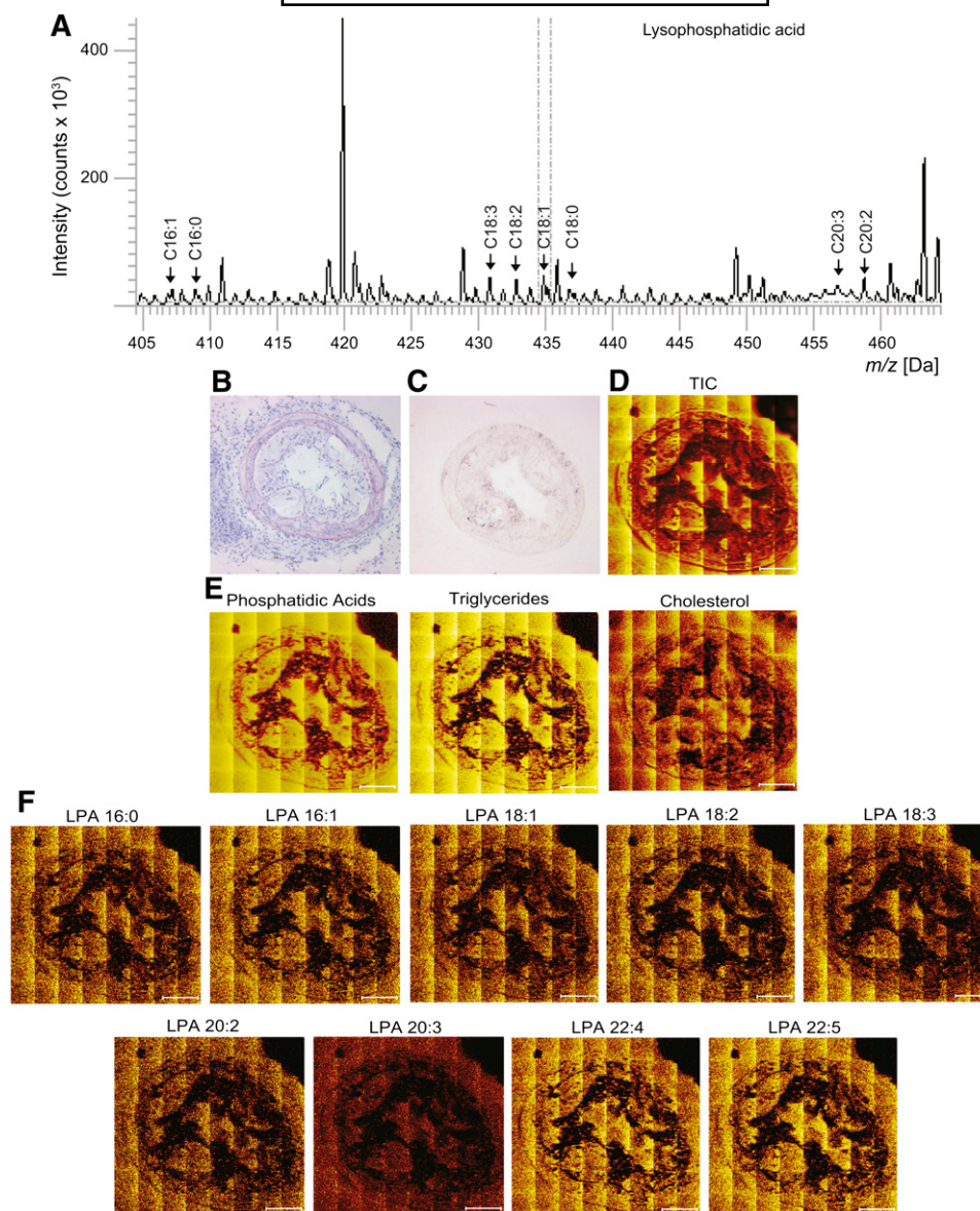
Fig. 1. A: TOF-SIMS spectra recorded from an atherosclerotic artery segment in negative mode with tentative peak assignments, showing LPA species. B: HE staining and C: MOMA-2 + macrophage staining of a mouse carotid artery lesion. Negative ion micrographs of a flanking lesion analyzed by TOF-SIMS. Color intensity corresponds to signal strength. D: Total ion current (TIC). E: Intraplaque distribution patterns of a selection of relevant ions including phosphatidic acids, triglycerides, and cholesterol. F: Several LPA species. Scale bar indicates 100 μm.
