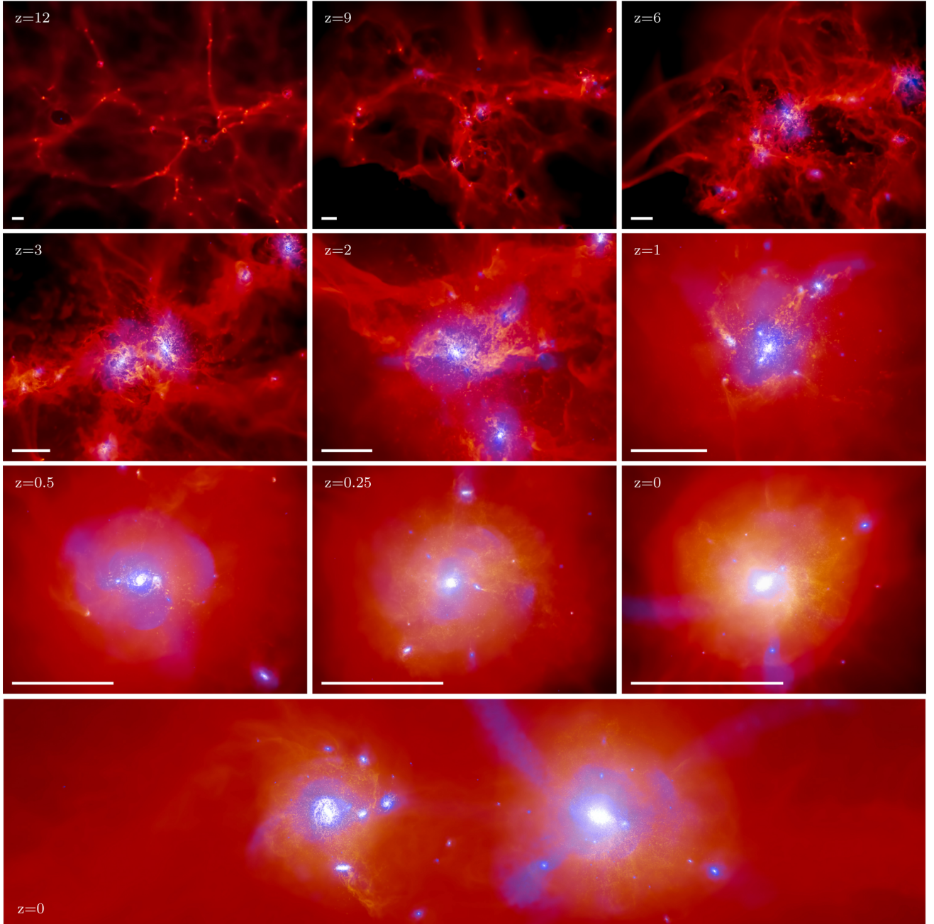
Figure 1. Top three rows: evolution of gas density (red colours) and stellar density (blue colours) in a comoving volume of side length 150 \times 200 \text{ h}^{-1} \text{ kpc} , centred on one of the main LG galaxies and its progenitors at resolution L1. For scale, a bar of length 100 \text{ h}^{-1} \text{ kpc} is shown on each panel. At z = 12 , before re-ionization, stars have already formed in some of the highest density regions, and feedback from supernovae has begun to blow bubbles into the gas. Over time stars form in many more haloes, and star-forming regions merge to form larger galaxies. By z = 1 , the main galaxy has formed, and continues to accrete both gas and satellites, many of which lose their gas on infall and are also tidally disrupted. At z = 0 , the central galaxy is surrounded by many satellite galaxies, and a complex stellar halo with visible shells and streams. Bottom row: slice through the entire LG in the same simulation.
