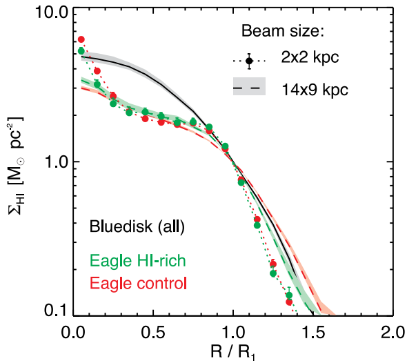
Figure E1. Variation of H I surface density profiles with beam size. The default low-resolution profiles with beam size 14 \times 9 \text{ kpc} FWHM (see Section 6) are shown with dashed lines, and the profiles obtained from higher-resolution maps with beam size 2 \times 2 \text{ kpc} FWHM as filled circles connected with dotted lines. In both cases, red represents control galaxies and green H I-rich galaxies. For guidance, the combined median Bluedisk profile is shown in black. Error bars indicate 1\sigma uncertainties on the median. Although there is some change in the detailed profile shape with increased resolution, the close match between H I-rich and control galaxies is robust to this change.
