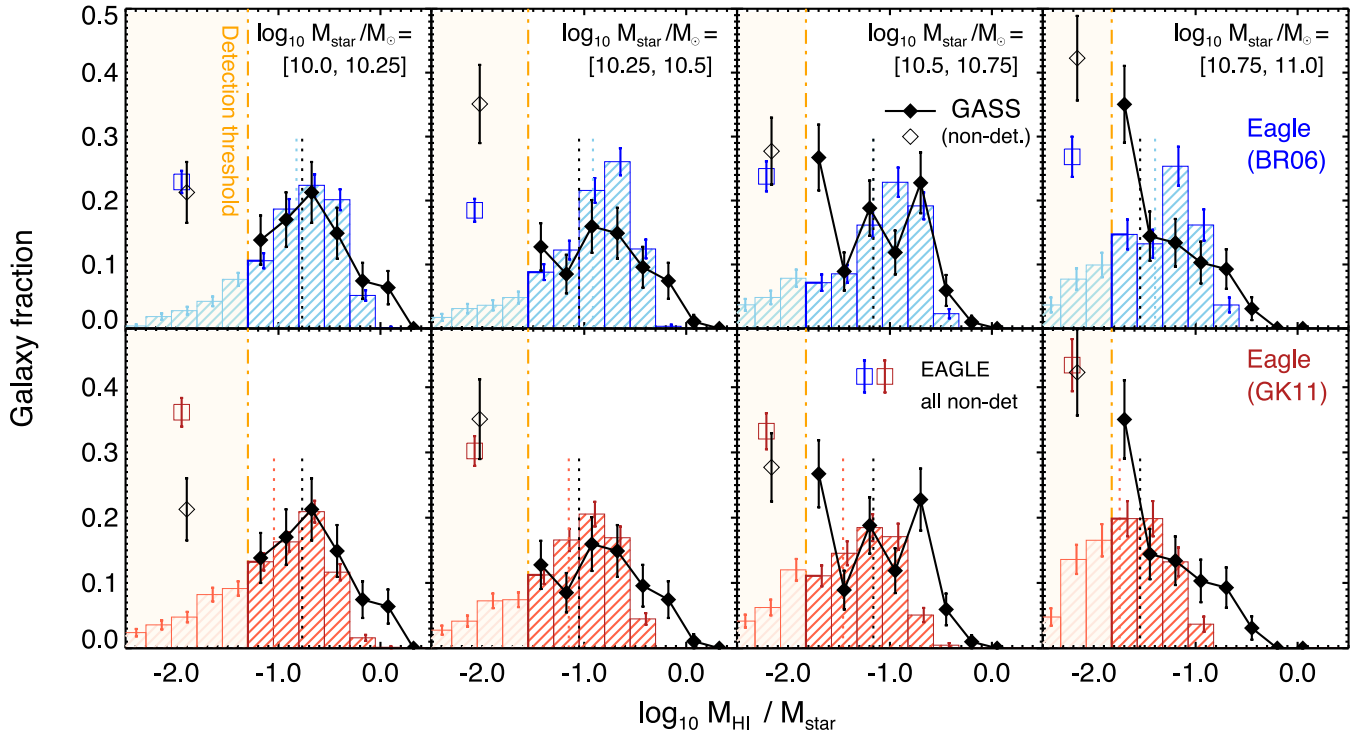
Figure 2. Comparison of the \text{H I} mass of EAGLE galaxies (blue/red histograms) with GASS observations (black lines); both samples include only central galaxies. In the top panel, the presence of \text{H}_2 in EAGLE is accounted for with the empirical Blitz & Rosolowski (2006) pressure-law prescription, while the bottom panel shows the corresponding results from the theoretical Gnedin & Kravtsov (2011) partition formula. The shaded region on the left is below the (maximum) GASS detection threshold in each panel; all simulated galaxies in this regime (light blue/red) are combined into the blue/red open square for comparison to the observations. Vertical black (blue/red) dotted lines indicate the median \text{H I} mass fraction of all GASS (EAGLE) galaxies per stellar mass bin; in the third panel of the top row both lie on top of each other. Error bars show statistical Poisson uncertainties. Both \text{H}_2 prescriptions lead to broad agreement of the predicted \text{H I} masses with observations, but the detailed match is considerably better for the Blitz & Rosolowski (2006) \text{H}_2 formula (top).
