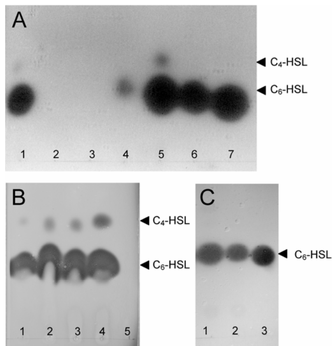
Fig. 3. C18-reverse phase thin-layer chromatography (TLC) analysis of N -acyl-L-homoserine lactones produced by Pseudomonas chlororaphis PCL1391 and mutant derivatives. A volume of 100 \mu l of a 72-h King's medium B culture supernatant of the strains was extracted with dichloromethane, and samples equivalent to 20 \mu l of culture supernatant were tested in the Chromobacterium TLC overlay assay. A , Autoinducer profiles of regulatory and biosynthetic mutants of P. chlororaphis PCL1391. Lane 1, PCL1391 wild type; lane 2, PCL1103 ( phzI ::Tn5luxAB); lane 3, PCL1104 ( phzR ::Tn5luxAB); lane 4, PCL1123 ( gacS ::Tn5luxAB); lane 5, PCL1111 ( psrA ::Tn5luxAB); lane 6, PCL1119 ( phzB ::Tn5luxAB); lane 7, synthetic N -hexanoyl-L-homoserine lactone (C 6 -HSL) standard (1 \times 10^{-10} mol). B , C 6 -HSL production by Pseudomonas chlororaphis PCL1391 and psrA mutant derivatives. Lane 1, PCL1391 wild type; lane 2, PCL1111 ( psrA ::Tn5luxAB); lane 3, PCL1140 ( phzI ::Tn5luxAB, psrA - ); lane 4, PCL1142 ( phzR ::Tn5luxAB, psrA - ); lane 5, PCL1139 ( psrA ::Tn5luxAB, gacS - ). C , C 6 -HSL production of the complemented P. ororaphis PCL1111 ( psrA ::Tn5luxAB). Lane 1, PCL1111 ( psrA ::Tn5luxAB); lane 2, PCL1111 harboring pMP6579 ( psrA ); lane 3, synthetic C 6 -HSL standard (1 \times 10^{-10} mol). Experiments were performed at least twice with similar results.
