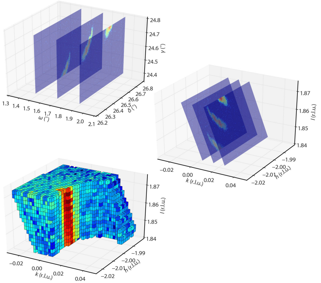
Figure 4.1. A graphical overview of the process performed by BINoculars . The data displayed here are a rocking scan through (h, k, l) = (-2, 0, 1.85) the diffraction pattern from a Pt(110) surface. Upper panel, raw data acquired by the 2D-detector with the corresponding angles \omega , \delta , \gamma from a six-circle diffractometer[68]. Middle panel, the diffractometer angles are mapped onto reciprocal space coordinates (h, k, l) . Lower panel, the averaged intensity of pixels on a regular grid of volumetric bins (voxels) is calculated. Part of the bins are removed for clarity. Note that the data in reciprocal space in the lower panel are constructed from a series of images over a larger range and with a denser sampling in \omega than shown in the other panels.
