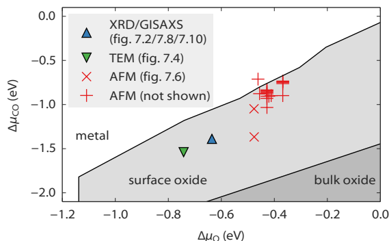
Figure 7.1. Experimental conditions of all experiments reported in this chapter, expressed in terms of the chemical potentials of carbon monoxide and oxygen. The three grey levels indicate three of the phases of a Pd(100) surface in contact with CO and O 2 , as calculated using DFT by Rogal et al[141]. Since a nanoparticle exposes multiple different facets, it is to be expected that the phase boundaries for a nanoparticle system will be in slightly different positions. The phase boundaries will also shift and blur because of the CO oxidation reaction itself[142]. The two triangles correspond to observed reaction oscillations, indicating that these points are near a phase boundary, whereas only microscopy images but no reactivity data could be obtained for the cross markers.
