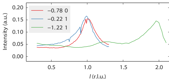
Figure 5.7. l -scans along the superstructure rods for the “0.22” reconstruction, taken at 150°C in pure NO at a total pressure of 200 mbar. The legend shows the h and k values of each scan. The intensity peaks strongly at integer l -values, meaning that the periodicity matches that of the bulk Pt lattice, suggesting that the reconstruction is some structure of Pt.
