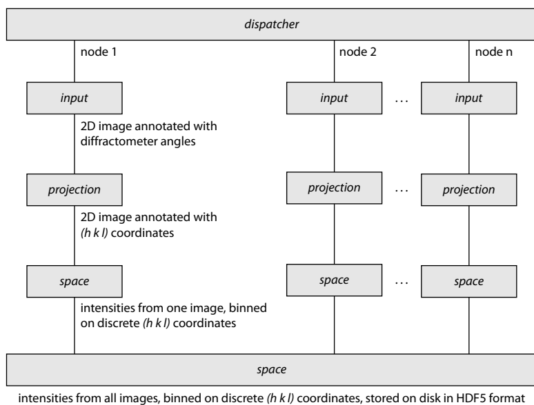
Figure 4.2. Block diagram of the process performed by BINoculars for a typical dataset from a diffraction experiment. The dispatcher distributes the load over multiple nodes from a computing cluster. The input class gathers the experimental data and calculates the diffractometer angles for each pixel. The projection class converts the angles to (h k l) coordinates. The intensities are binned on a discrete grid by the space class, and finally the intermediate results from each node are combined into a single space .
