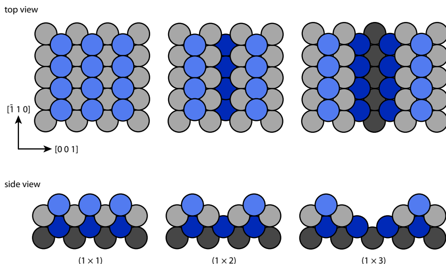
Figure 5.1. Ball models of the surface structure of Pt(110), without a reconstruction (left) and with the (1 \times 2) and (1 \times 3) missing-row reconstructions (middle and right)[96]. The h -axis of reciprocal space is chosen to correspond to the closed-packed [1\bar{1}0] direction and k to the open [001] direction.
