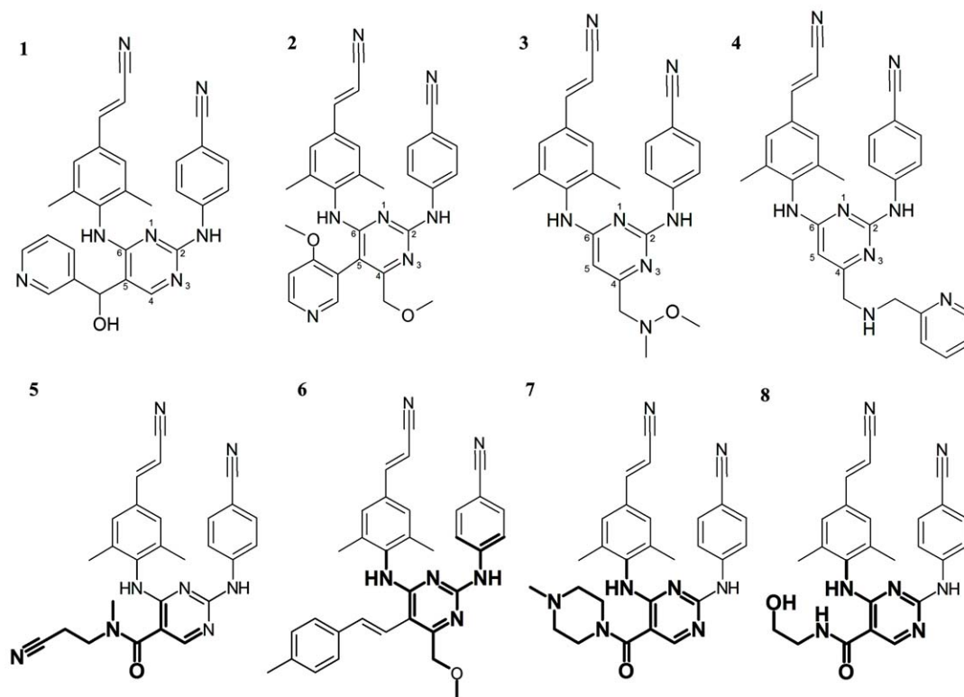
Figure 6. Example structures that were included in the model. A selection of both compounds containing accurately (1,2) and inaccurately modeled chemistry (3,4). Also shown are compounds containing a substructure positively correlated with pEC_{50} (5,6) and compounds containing a substructure negatively correlated with pEC_{50} (7,8). In the upper part, shown are sample compounds that were accurately predicted using the LOSO models, a low RMSE (1, RMSE was 0.22 log units, R_0^2 was 0.96) and a high R_0^2 (2, R_0^2 was 0.89, RMSE was 0.26). Secondly, sample compounds that were predicted inaccurately using the LOSO models, a high RMSE (3, RMSE was 1.12 log units, R_0^2 was -0.10 ) and a low R_0^2 (4, R_0^2 was -3.66 , RMSE was 0.61). The lower part shows the 17 th best substructure (5) and the 30 th best substructure (6). Conversely the 3 rd worst substructure (7) and the 4 th worst substructure (8) are depicted.
