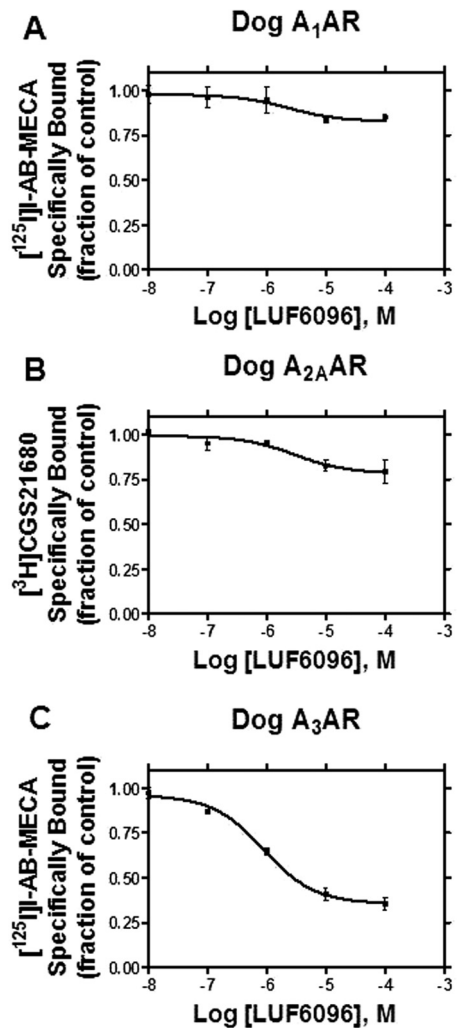
Fig. 5. Effect of LUF6096 on equilibrium orthosteric radioligand binding to the canine A 1 (A), A 2A (B), and A 3 (C) ARs. Membranes (50 \mu g) were incubated with [ 125 I]I-AB-MECA ( \sim 0.5 nM; A 1 and A 3 ARs) or [ 3 H]CGS21680 ( \sim 10 nM; A 2A ARs) for 2 h at room temperature in the presence of increasing concentrations of LUF6096. Nonspecific binding was determined with 200 \mu M adenosine-5'-N-ethylcarboxamide. The data shown are representative of three independent experiments.
