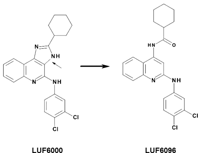
Fig. 1. Chemical structures of the PAMs of the A_3 AR, LUF6000 (left) and LUF6096 (right). The arrow points to the bond deleted in LUF6000 that led to LUF6096.
