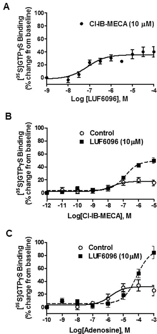
Fig. 4. Effect of LUF6096 on [ 35 S]GTP \gamma S binding in assays with the canine A 3 AR. Incubations were started by the addition of the membrane suspension (5 \mu g of protein) as described under Materials and Methods and carried out in quadruplicate for 2 h at 25°C. The membrane solutions were preincubated with LUF6096 for 30 min at 25°C before the addition of \sim 0.1 nM [ 35 S]GTP \gamma S. A, the effect of increasing concentrations of LUF6096 on [ 35 S]GTP \gamma S binding in response to a maximal concentration of Cl-IB-MECA (10 -5 M) ( n = 9). B, stimulation of [ 35 S]GTP \gamma S binding by increasing concentrations of Cl-IB-MECA in the absence (control) or presence of LUF6096 (10 \mu M) ( n = 6). C, stimulation of [ 35 S]GTP \gamma S binding in response to increasing concentrations of adenosine in the absence (control) or presence of LUF6096 (10 \mu M) ( n = 5).
