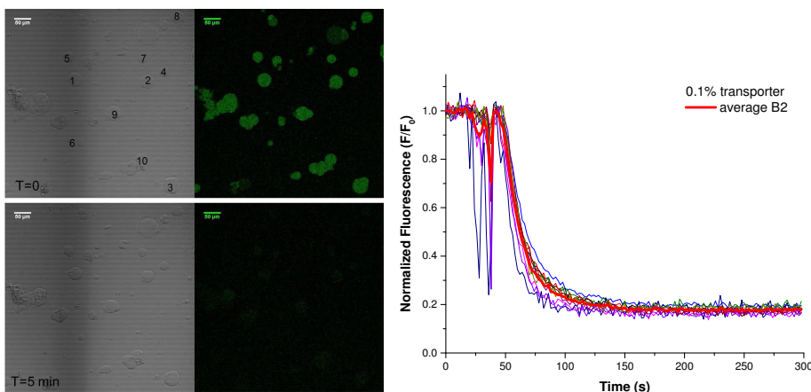
Figure A4. Bright-field and fluorescence microscopy images before (top) and after (bottom) addition of NaCl to GUVs containing 0.1% transporter ( experiment B2 ). The normalized fluorescence intensity over time is given for the individual numbered GUVs and for the average of all numbered GUVs (fat red line). The average diameter of the GUVs used for the average trace is 36 \mu\text{m} .
