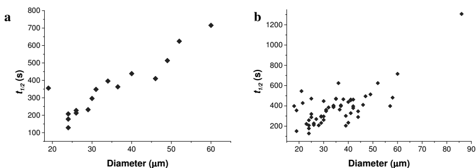
Figure 6. Plot of the half-lives (from single exponential fits, experiments with 0.01% transporter) versus the diameter of 16 individual GUVs from one experiment ( a ) and from 56 GUVs of 6 experiments combined in one graph ( b ).
