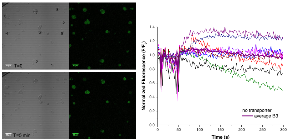
Figure A1. Bright-field and fluorescence microscopy images before (top) and after (bottom) addition of NaCl to GUVs without transporter ( experiment B3 ). The normalized fluorescence intensity over time is given for the individual numbered GUVs and for the average of all numbered GUVs (fat purple line). The average diameter of the GUVs used in the average trace for 36 \mu\text{m} .
