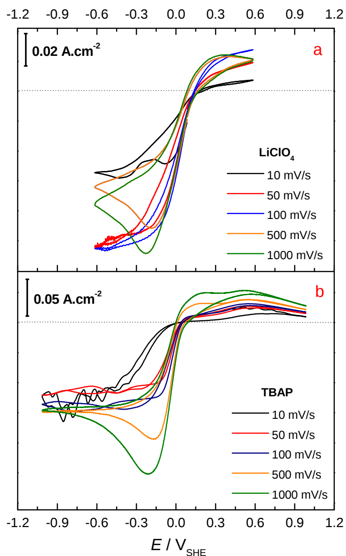
Figure A2. Cyclic voltammeteries for a polycrystalline platinum wire in acetonitrile, in presence of 10 mM \text{HClO}_4 , under hydrogen atmosphere. The second cycle is shown for each scan rate. a) 100 mM \text{LiClO}_4 or b) 100 mM TBAP, as supporting electrolytes. The horizontal dotted lines mark zero current.
