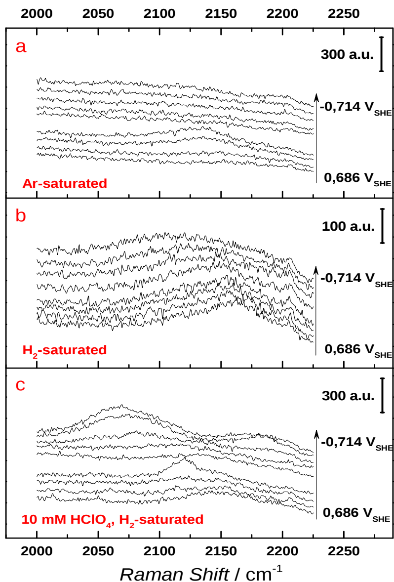
Figure 8. Potential-dependent SER spectra for acetonitrile, containing 100 mM LiClO 4 as supporting electrolyte: a) Argon atmosphere; b) Hydrogen atmosphere; c) After adding 10 mM HClO 4 ; hydrogen atmosphere.
