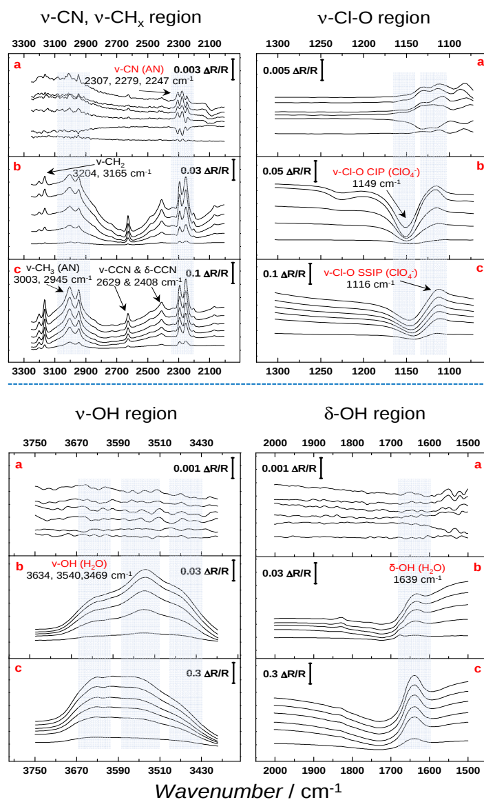
Figure 6. Potential-dependent SNIPTIR spectra for a polycrystalline platinum electrode in acetonitrile, containing 100 mM LiClO 4 as supporting electrolyte: a) Argon atmosphere; b) Hydrogen atmosphere; c) After adding 10 mM HClO 4 under hydrogen atmosphere. Reference spectrum: -0.500 V Ag 0 /Ag + (corresponding to -0.314 V SHE ).
