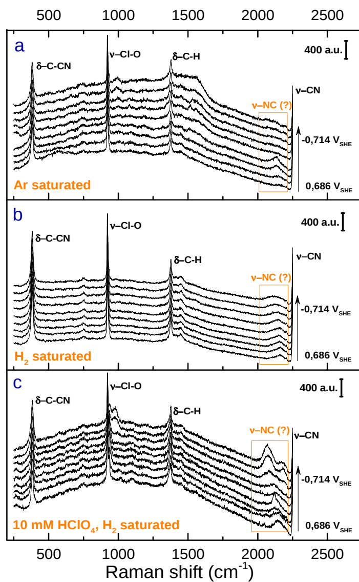
Figure A3. SERS spectra for acetonitrile, containing 100 mM LiClO 4 as supporting electrolyte.
