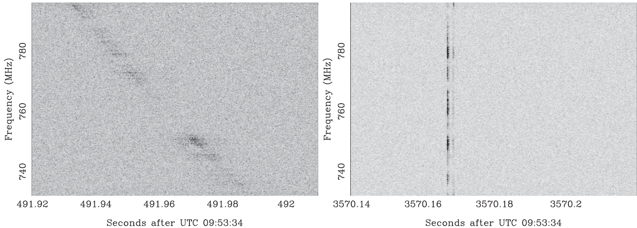
Figure 8. Example pulses occurring when the pulsar is in the weak state. The left-hand pulse originated at the pulsar. The right-hand pulse was caused by RFI.
