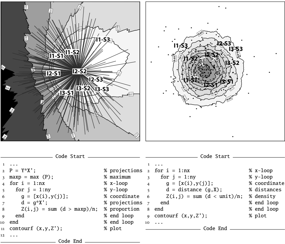
Figure 5.6 PCA solution (left-hand panel) and landscape segmentation analysis solution (right-hand panel) for the tomato soup data with first choice contours and corresponding MATLAB code.
