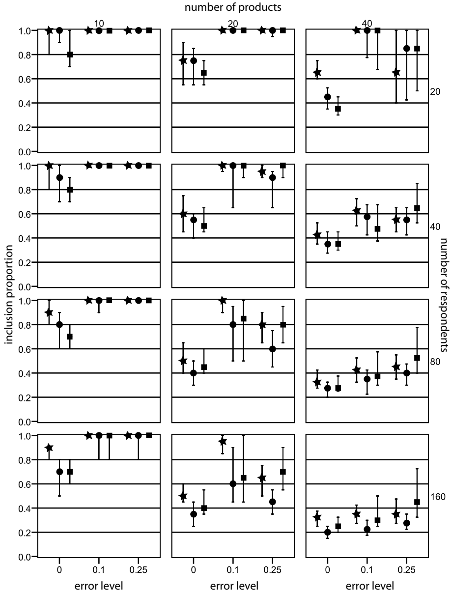
Figure 6.4 High-low graphs for inclusion proportions when data are missing by researcher, where the I-beams (low-close-high) indicate 95% chances on minimal values for \phi_{xy} (.95-.98-.99), \phi_y (.95-.98-.99), and \tau_b (.70-.80-.90), indicated by stars, dots and squares, respectively.
