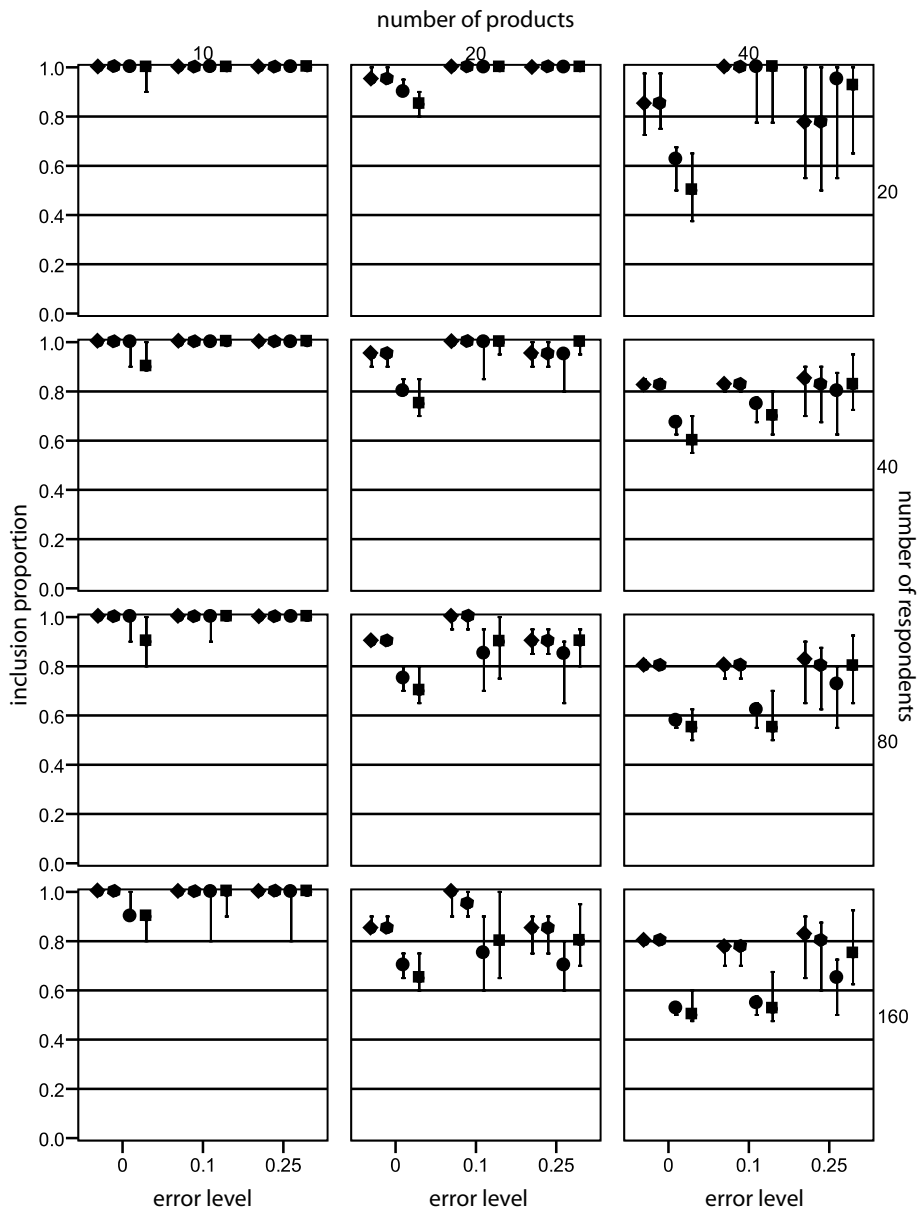
Figure 6.5 High-low graphs for inclusion proportions when data are missing by respondent, where the l-beams (low-close-high) indicate 95% chances on minimal values for \phi_{xy}^{high} (.95-.98-.99), \phi_{xy}^{low} (.95-.98-.99), \phi_y (.95-.98-.99), and \tau_b (.70-.80-.90), indicated by diamonds, polygons, dots and squares, respectively.
