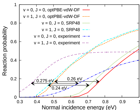
FIGURE 6.5 Reaction probability as a function of normal incidence energy for ( \nu = 0 , J = 0 ) D_2 and ( \nu = 1 , J = 0 ) D_2 dissociating on Cu(111) for the SRP48 and optPBE-vdW-DF functionals. \Delta E_0 at a reaction probability of 15% are indicated. Experimental data for T_s = 925 K by MICHELSEN et al. , 73 reanalysed by NATTINO et al. 77
